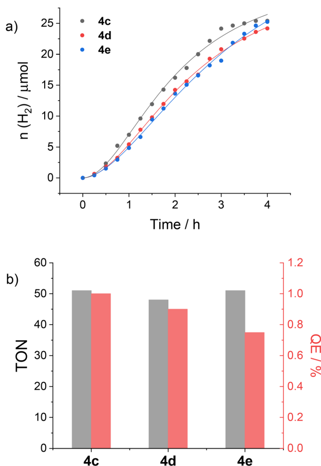
Fig. 5 (a) Kinetics of hydrogen evolution upon irradiation (460 nm LED) of 1 M acetate buffer (pH 5) solutions containing 0.5 mM [Ru(bpy) 3 ] 2+ , 0.1 M ascorbic acid and 0.1 mM 4c–e ; (b) maximum TONs and QEs.
