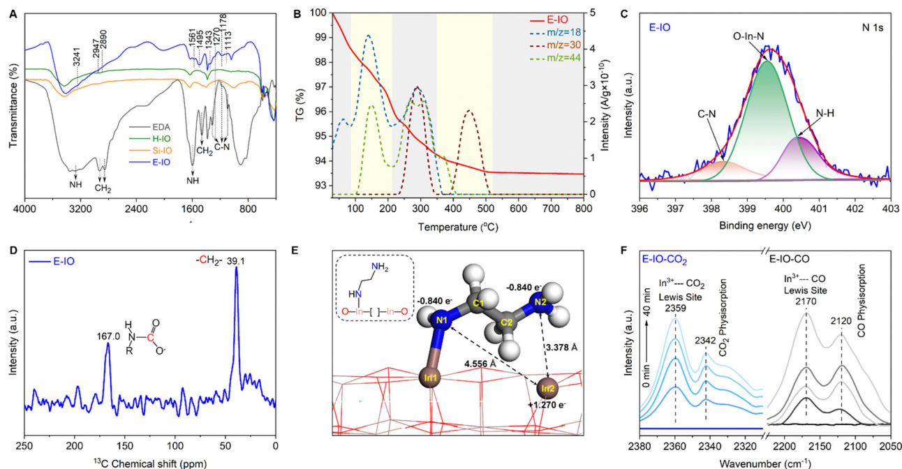
Fig. 2 Characterization of samples (A) FTIR spectra of H-IO, Si-IO and E-IO. (B) TGA-MS curves of E-IO in air condition. (C) High resolution N 1s XPS spectra of E-IO. (D) ^{13}\text{C} MAS NMR spectra of E-IO at room temperature. (E) Optimized structure of the grafting state \text{InNH}_2 \cdot \text{In} . (F) In situ DRIFTS spectra of the adsorption of \text{CO}_2 (left) and CO (right) on the E-IO surface at 298 K.
