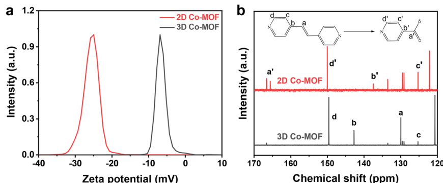
Fig. 4 (a) Zeta potential of the 3D Co-MOF precursor and 2D Co-MOF nanosheets; (b) the ^{13}\text{C} NMR spectra of the solvents derived from 3D Co-MOF precursor and 2D Co-MOF nanosheet.
