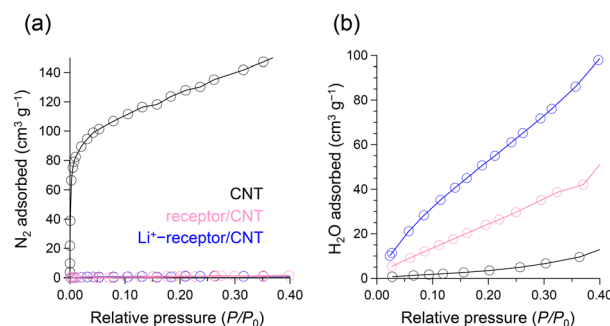
Fig. 3 (a) \text{N}_2 adsorption isotherms at 77 \text{ K} . (b) Water–vapor adsorption isotherms at 298 \text{ K} .
