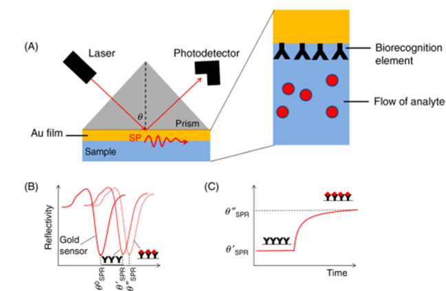
Fig. 5 Example of SPR sensing technology. As the analyte binds onto the sensor's surface (a), a shift in the incident angle for SPR is noted (b), indicating that the analyte is present. As more analyte binds, the change in angle levels off (c). 37 This figure has been modified from its original publication.
