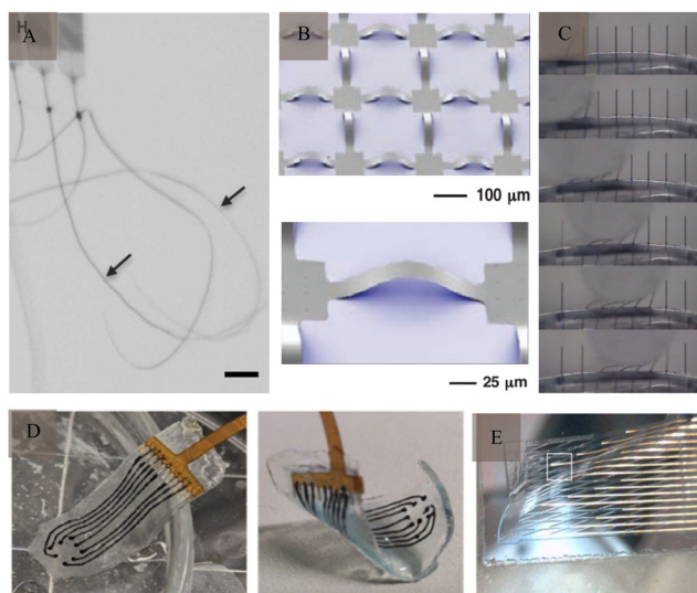
Fig. 6 Flexible electrodes. (A) Ultraflexible nanoelectronic probes, arrows indicate the probes (scale bar: 100 \mu m). Reproduced with permission from ref. 59. (B) Stretchable silicon membrane integrated on elastomeric substrates and enlarged image. Reproduced with permission from ref. 60. (C) Silicone-embedded carbon fibres in bend test. Reproduced with permission from ref. 61. (D) Viscoelastic array made of hydrogel (scale bar: 3 \mu m). Reproduced with permission from ref. 71. (E) A mesh electrode after being released from its silicon wafer. Reproduced with permission from ref. 62.
