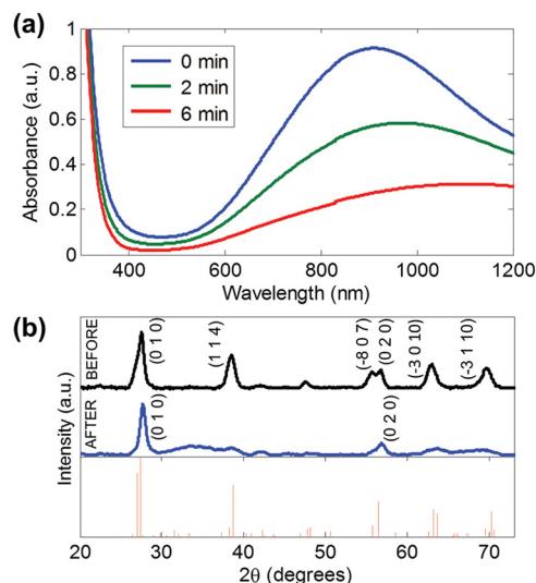
Fig. 20 (a) UV-vis-NIR absorption spectra of WO 2.83 nanorods in N -methylpyrrolidone upon heating at 175 °C in air for 0, 2, and 6 min. (b) XRD patterns of WO 2.83 nanorods in N -methylpyrrolidone (top) before and (middle) after heating at 175 °C for 6 min in air and (bottom) the reference pattern for WO 2.83 . Reproduced from ref. 15 with permission from ACS, copyright 2012.
