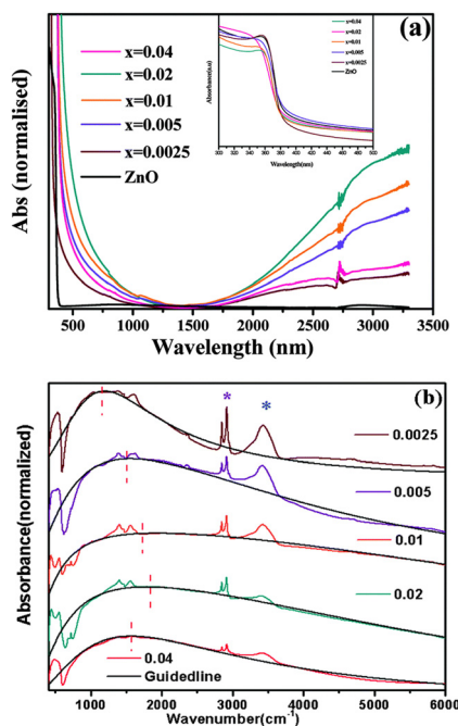
Fig. 18 (a) Optical absorption spectra of pure ZnO and doped Zn 1-x Ga x O nanocrystals in the vis-NIR region. The inset depicts the band-gap absorption of the samples. (b) FTIR spectra of doped samples showing the plasmonic NIR absorption. Additional sharp peaks (asterisks) arise from the organic ligand oleylamine absorbed on the nanocrystal surface. Blue and purple asterisks represent N–H stretching and symmetric/asymmetric stretching vibration of long hydrocarbon chains, respectively. The black dotted line and the red vertical dotted line are guiding lines for the shifting of plasmonic absorption. Reproduced from ref. 61 with permission from RSC, copyright 2015.
