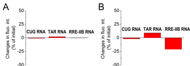
Fig. 2 Structures of the CUG RNA, HIV-1 TAR RNA and HIV-1 RRE-IIB RNA oligonucleotides used in this study and changes in the fluorescence intensity (in% of the initial intensity) of aurones ( A ) 2a and ( B ) 1d ( c_{\text{lig}} = 5 \mu\text{M} ) in the presence of 1 equiv. of each RNA oligonucleotide in a buffer (pH = 7); positive values indicate fluorescence light-up in the presence of RNA and negative values indicate fluorescence quenching in the presence of RNA. The fluorescence output was measured upon excitation at \lambda_{\text{ex}} = 350 \text{ nm} for 2a and at \lambda_{\text{ex}} = 450 \text{ nm} for 1d . To ensure the reproducibility, each measurement was repeated at least three times, and the repeat experiments gave values within 20%.
