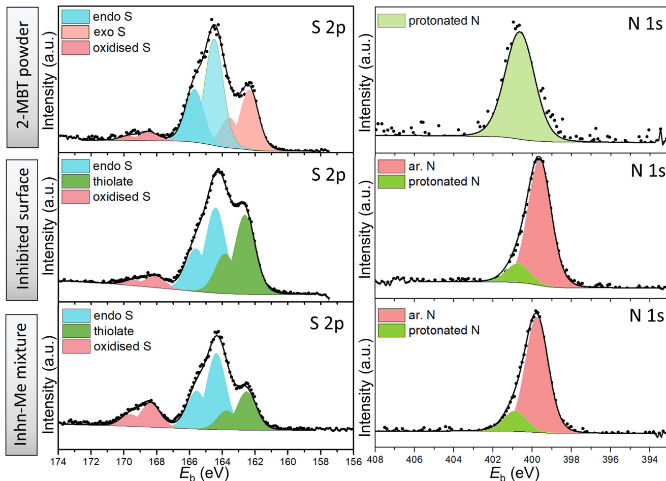
Fig. 6 High-resolution XPS spectra of S 2p and N 1s of 2-MBT powder (reference), ZE surface treated with 2-MBT and precipitates of inhibitor solution mixed with \text{ZnCl}_2 .
