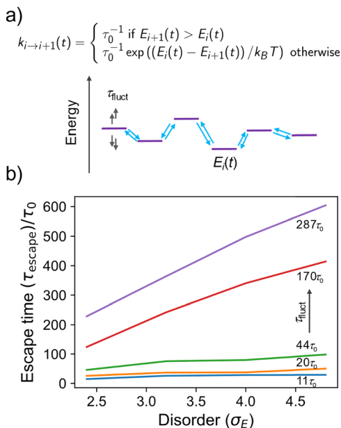
Fig. 4 (a) Schematic of a 1D kinetic model with nearest neighbour hopping where the on-site energy fluctuates with characteristic time \tau_{\text{fluct}} and the characteristic hopping time is \tau_0 . (b) Escape time (defined in text) of a charge carrier as a function of the disorder \sigma_E for different values of fluctuation time \tau_{\text{fluct}} = 11, 20, 44, 170 and 287 \tau_0 .
