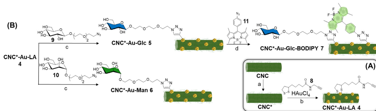
Scheme 1 (A) Synthesis of CNC*-Au-LA 4 . Reaction conditions: a. Sulfur trioxide pyridinium complex, dimethyl sulfoxide, 4 h, 25 °C; b. HAuCl 4 , NaBH 4 , water:methanol (1 : 9), and 8 . (B). Synthesis of CNC*-Au-Glc 5 , CNC*-Au-Man 6 , and CNC*-Au-Glc-BODIPY 7 . Reaction conditions for c and d: CuSO 4 , sodium ascorbate (water for c and DMF for d), overnight, room temperature.
