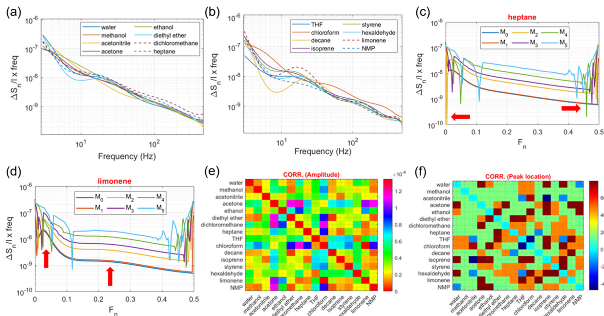
Fig. 4 (a) and (b) Differential spectral noise obtained for the tested VOCs by subtraction with the spectral noise measured for nitrogen. (c) Spectral components ( M_0 to M_5 ) obtained after the application of the filter bank to the differential noise measured for heptane. (d) Similar spectral components obtained for limonene. Note: the red arrows mark some visual differences between the traces of the spectral components for heptane and limonene. (e) Correlation matrix for the tested VOCs in terms of the sum of the differences in peak intensity measured for different spectral components. (f) Similar correlation matrix calculated in terms of the average difference in peak location measured for M_0 to M_5 .
