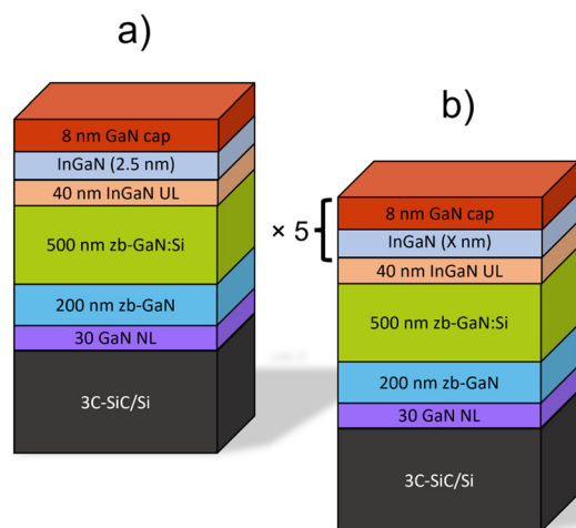
Fig. 1 Diagram of (a) zb-SQW and (b) MQW samples used in this study.
