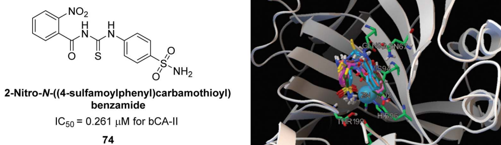
Fig. 26 Chemical structure of compound 74 and its IC_{50} value against bCA-II along with its docking image.
