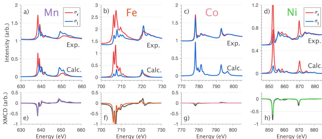
Fig. 8 Normal incidence ( \vec{E} \perp \vec{c} ) single crystal L_{2,3} -edge XMCD measurements and calculations of \text{Li}_2(\text{Li}_{1-x}\text{TM}_x)\text{N} (where TM = Mn, Fe, Co and Ni). (a–d) Circular polarisation absorption spectra \sigma_r (red) and \sigma_l (blue) with resultant (e–h) XMCD ( \sigma_r - \sigma_l ) spectra; experimental (black) and charge-transfer multiplet calculations (colour) measured at 21 K and 14 T.
