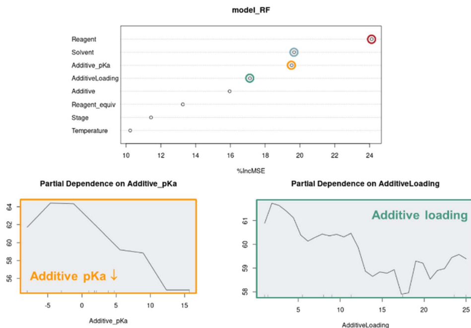
Fig. 12 Random forest (RF) model of the combined autonomous optimization data ranking of parameter influences and partial dependence plots of predicted product 2 UPLC area % on additive \text{pK}_\text{a} and loading.
