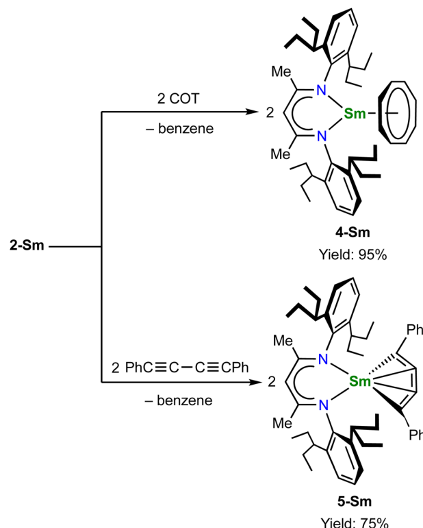
Scheme 2 Reactivity of 2-Sm as a four-electron reductant.
