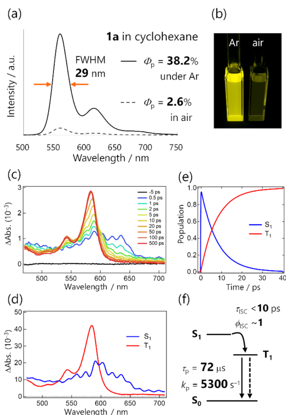
Fig. 2 (a) Steady-state photoluminescence spectra of 1a in cyclohexane ( 4.4 \times 10^{-6} \text{ M} , excited at 368 nm). (b) Photograph of solutions of 1a under 365 nm excitation. (c) fs transient absorption spectra of 1a in cyclohexane excited at 355 nm. (d and e) Selected results from the global analysis based on a sequential model; (d) evolution-associated spectra and (e) corresponding concentration kinetics. Coherent artefact signals are omitted for clarity. (f) Schematic summary of the excited-state dynamics in 1a .
