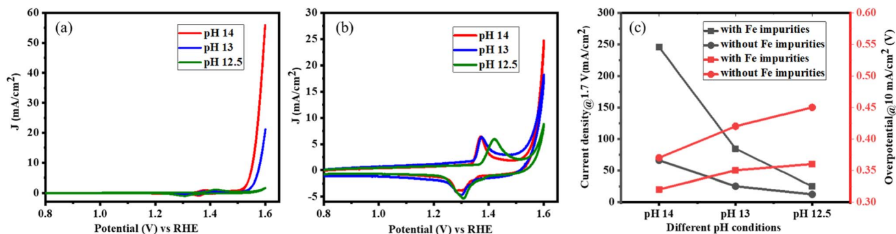
Fig. 7 Cyclic voltammetry data after the 50 th cycle was obtained for \text{LaNiO}_3 under different pH conditions: (a) with Fe impurities, (b) without Fe impurities, (c) overview of the overpotential at 10 \text{ mA cm}^{-2} and current density at 1.7 \text{ V} vs. RHE at different pH conditions with and without Fe impurities in the electrolyte.
