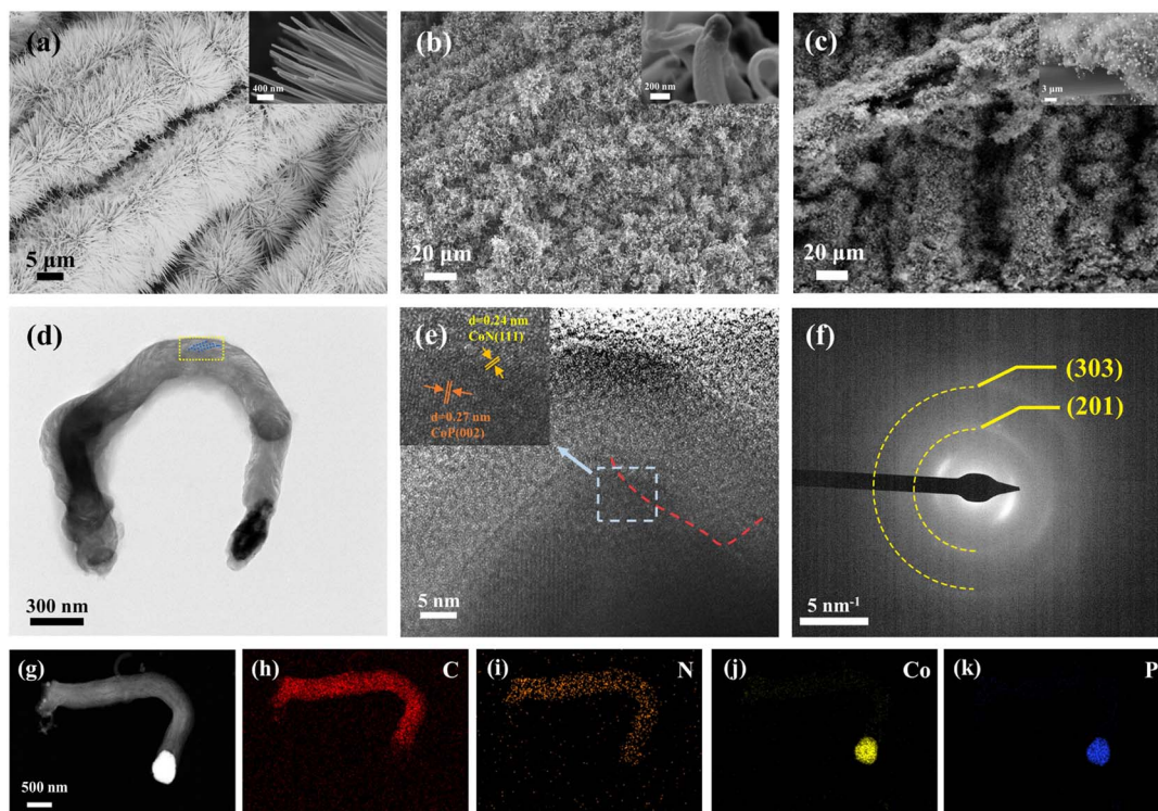
Fig. 2 (a) SEM images of \text{Co}(\text{CO}_3)_x\text{OH}/\text{CC} nanoneedle arrays. Inset: details of the nanoneedle arrays, (b) SEM of \text{Co@NCNRs/CC} and the inset shows the details of single \text{Co@NCNR} , and (c) SEM of \text{CoP/CoN@NCNRs/CC} ; (d) TEM and (e) HR-TEM. Inset: lattice spacing of \text{CoP} and \text{CoN} , (f) SAED pattern, and (g–k) compositional elemental mapping of \text{CoP/CoN@NCNRs/CC} .
