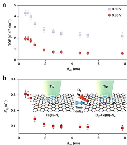
Fig. 22 (a) The imaging of TOF at 0.85 and 0.80 V, (b) time-delay SI-SECM titration imaging and the reaction rate constant ( k' of O 2 ) for O 2 binding on Fe(III)-N 4 sites. Reproduced from ref. 93 with permission from Springer Nature, copyright 2021.
