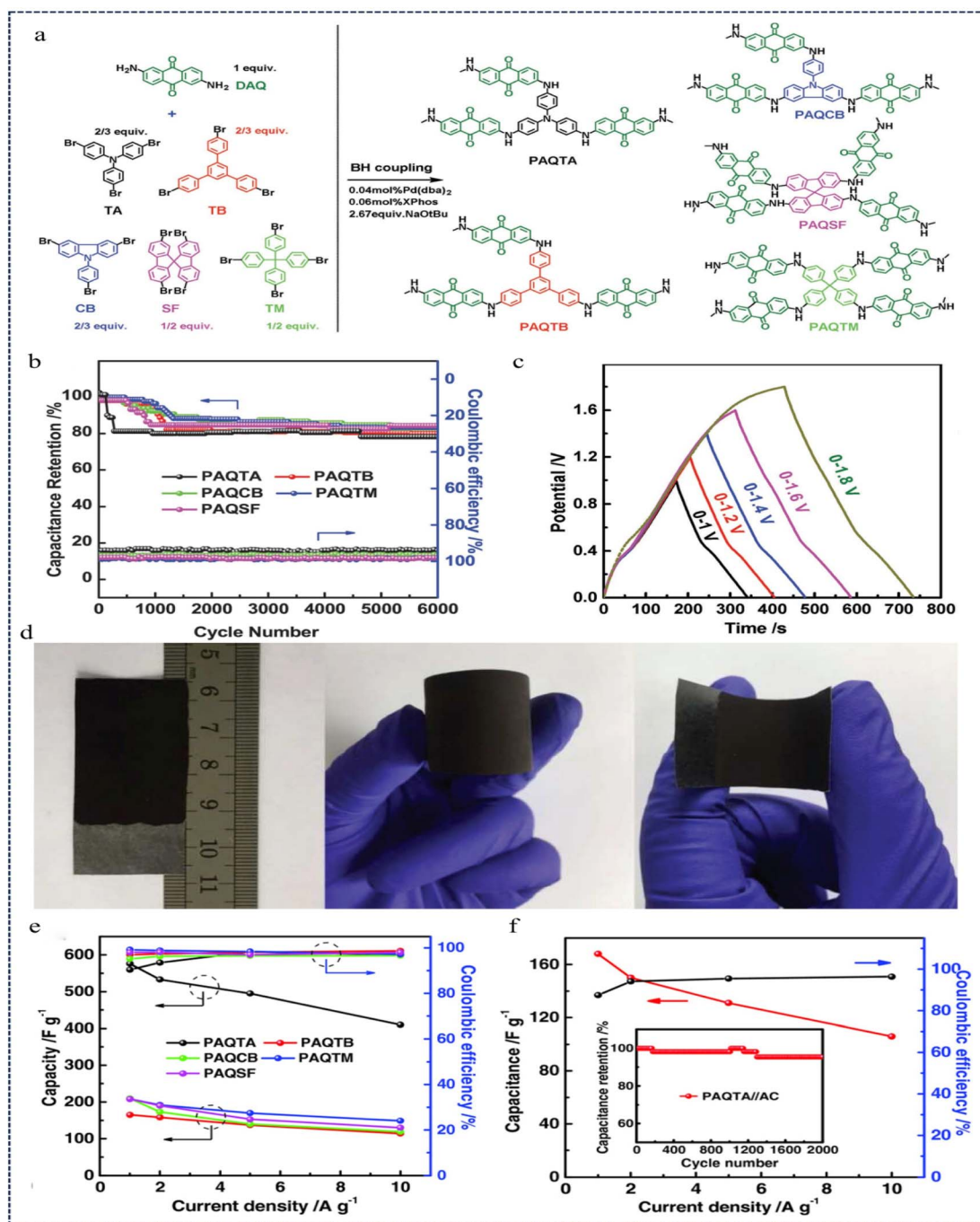
Fig. 20 (a) Synthetic routes of PAQTA, PAQTB, PAQCB, PAQSF, and PAQTM. (b) Cyclability tests and coulombic efficiencies of PAQTs. (c) GCD curves at a current density of 1.0 \text{ A g}^{-1} . (d) Photographs of flexible PAQTA electrodes and electrochemical performance of PAQTs obtained in 0.5 \text{ M H}_2\text{SO}_4 . (e) Specific capacitance and coulombic efficiency of PAQTs obtained at different current densities. (f) Specific capacitance and its retention as well as the coulombic efficiency based on the total mass of the two electrodes versus current density with the inset showing the cycle durability of the device at a current of 2.0 \text{ A g}^{-1} . 126 Copyright 2018, Wiley.
