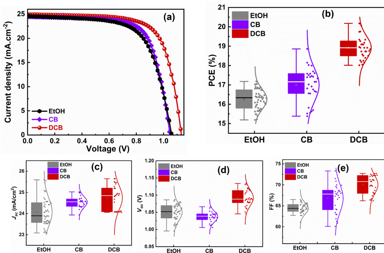
Fig. 4 (a) Current density–voltage ( J - V ) characteristics of the champion devices treated using EtOH, CB, and DCB antisolvents with device area of 0.092 cm 2 . (b) Frequency distribution plot of the planar heterojunction perovskite solar cells (PSCs) treated with corresponding anti-solvents (b) power conversion efficiency (PCE) showing DCB-treated PSCs averaging efficiencies 11% and 16% higher than those of CB- and EtOH-treated PSCs respectively, (c) short-circuit current density, ( J sc ) with marginally similar average currents between DCB- and CB-treated PSCs (d) open-circuit voltage ( V oc ) showing DCB-treated PSCs averaging values of 3–5% higher than those of CB- and EtOH-treated PSCs, (e) fill-factor (FF) showing DCB-treated PSCs averaging values 4% and 11% higher than those of CB- and EtOH-treated PSCs respectively.
