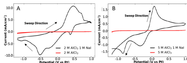
Fig. 2 Cyclic voltammograms (CVs) for EMIM[TFSI] electrolyte as affected by \text{AlCl}_3 and NaI. CVs shown for (A) 2 M \text{AlCl}_3 with and without 1 M NaI and (B) 5 M \text{AlCl}_3 with and without 1 M NaI. CVs were collected using a 3 mm Ni disk at 100 \text{ mV s}^{-1} with a platinum (Pt) wire quasi-reference electrode and a Pt wire counter electrode.
