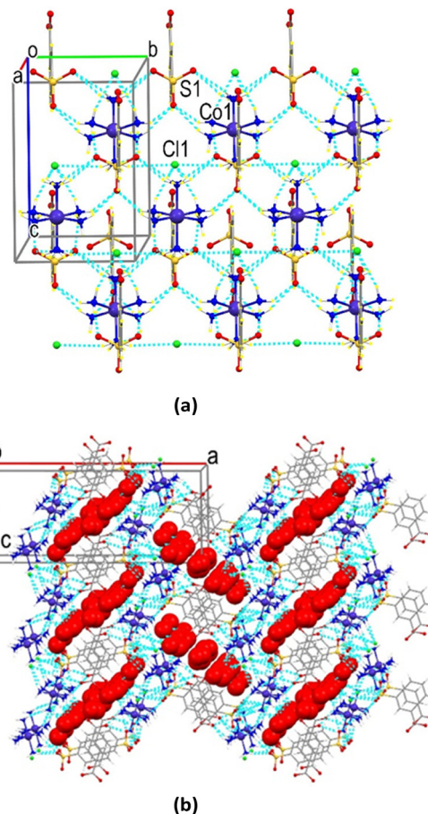
Fig. 3 (a) A fragment of the supramolecular layer in which the [\text{Co}(\text{NH}_3)_6]^{3+} cations are linked by H-bonds with the \text{Cl}^- anions and oxygen atoms of the sulfonate groups in 3 . (b) Formation of channels in the crystal due to bridging of layers by \text{N-H}\cdots\text{O} bonds of sulfonate and carboxylate groups of 3-sb . The solvent water molecules are shown in a space-filling mode, and hydrogen bonds are depicted as blue dashed lines.
