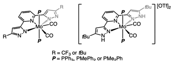
Fig. 1 Overview of the new heptacoordinated Mo(II) complexes described in this article.
