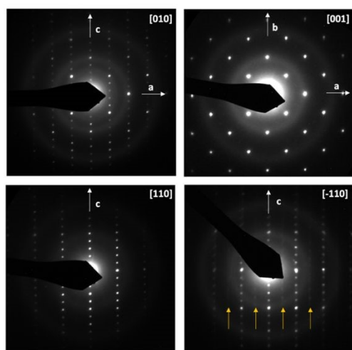
Fig. 2. Electron diffraction patterns of \text{Eu}_3\text{Ta}_2\text{ON}_5 along [010] , [001] and [110] axes. Orange arrows indicate superstructure reflections observed in some crystals, that can be indexed in a \sqrt{2}a_0 \times \sqrt{2}a_0 \times c_0 unit cell.
