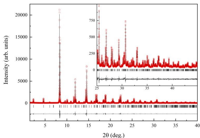
Fig. 1. Rietveld fit to synchrotron X-ray powder diffraction data ( \lambda = 0.41376 \text{ \AA} ) of \text{Eu}_3\text{Ta}_2\text{ON}_5 , performed in the I4/mmm space group with a = 3.98240(1) , c = 20.42020(6) \text{\AA} . The inset shows the high 2\theta region enlarged.
