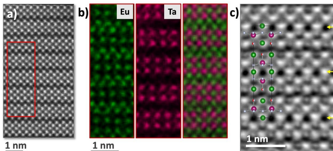
Fig. 3. (a) HAADF-STEM image of a \text{Eu}_3\text{Ta}_2\text{ON}_5 crystal along the [010] zone axis. The image shows a n=2 Ruddlesden-Popper structure, with two perovskite blocks intergrowing with a rock salt-type layer. The inset shows the corresponding area for the elemental EDX maps. (b) From left to right, atomic resolution EDX maps of Eu (in green), Ta (in magenta) and a combined colour map. (c) iDPC image with the \text{Eu}_3\text{Ta}_2\text{ON}_5 structure overlay (Eu: green, Ta: magenta, O: red and N: white). Yellow arrows point to the planes in which the anion vacancies are located.
