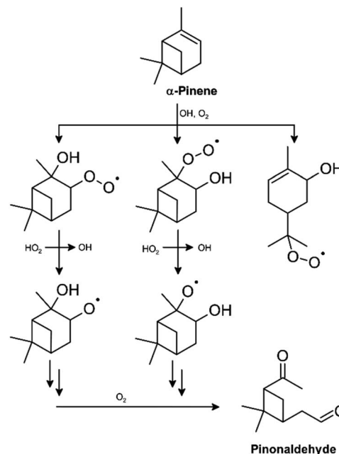
Fig. 3 OH production via the reaction of \alpha -pinene-derived peroxy radicals with HO 2 , as suggested by Eddingsaas et al. 37
