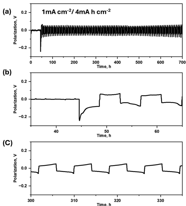
Fig. 1 Li metal symmetric cell cycling: (a) voltage profiles during lithium plating/stripping processes in Li|Li symmetrical cells containing 30 mol% LiTFSI in P 1111 FSI electrolytes at current density 1.0 mA cm -2 (4 mA h cm -2 ), at 50 °C (b) and (c) are the zoomed view.
