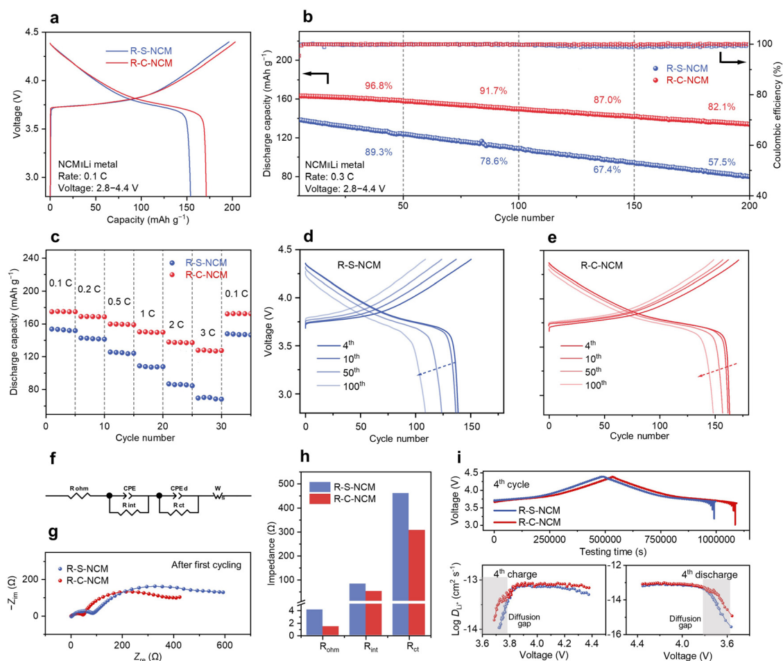
Fig. 4 Electrochemical deterioration for the regenerated NCM cathodes with impurity residue. (a) Initial galvanostatic charge–discharge curves of R-S-NCM and R-C-NCM at 0.1C ( 1C = 150 \text{ mA h g}^{-1} ) and (b) long cycling test and capacity retention in a half-cell. (c) Rate capabilities of R-S-NCM and R-C-NCM. Charge–discharge curves of (d) R-S-NCM, (e) R-C-NCM in the voltage range of 2.8–4.4 V (vs. Li/Li^+ ) at different cycles. (f) Equivalent circuit applied in the EIS measurements. Nyquist plots of (g) R-S-NCM and R-C-NCM and (h) fitting results showing the Ohmic resistance ( R_{ohm} ), interface resistance ( R_{int} ), and charge-transfer resistance ( R_{ct} ). (i) GITT curves and the calculated Li^+ -diffusion rate of R-S-NCM and R-C-NCM for the 4th cycle number after activation in the same charge–discharge period. The shadow area indicates low Li^+ diffusion in a certain voltage range.
