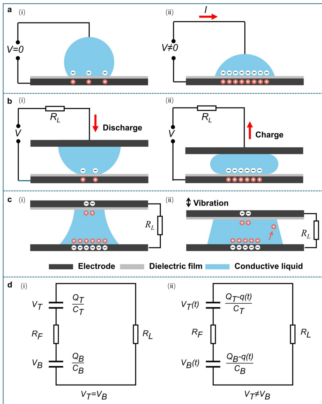
Figure 3. Basic working principles and equivalent circuit diagram. a) Working principle of the EWOD process. (i) no external voltage applied between the metal and the electrolyte solution, (ii) external voltage applied between the metal and the electrolyte solution. b) Working principle of the REWOD process. c) Working principle of the water bridge REWOD process. d) Equivalent circuit diagram of the water bridge REWOD process.
