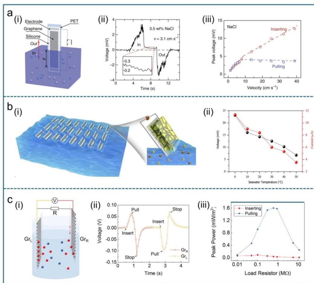
Figure 22. Application of waving energy generator. a) (i) The graphene is placed on a PET substrate and moved vertically on the water surface in the container to generate waving potential. a) (ii) The voltage signals generated when the sample is inserted and pulled out of a 0.6\text{ M} NaCl solution at a speed of v = 3.1\text{ cm/s} . a) (iii) The relationship between the magnitude of the positive peak voltage and the negative peak voltage and the speed at which graphene moves across the surface of a 0.6\text{ M} NaCl solution. Reproduced with permission. 275 Copyright 2014, Springer Nature. b) (i) The schematic
