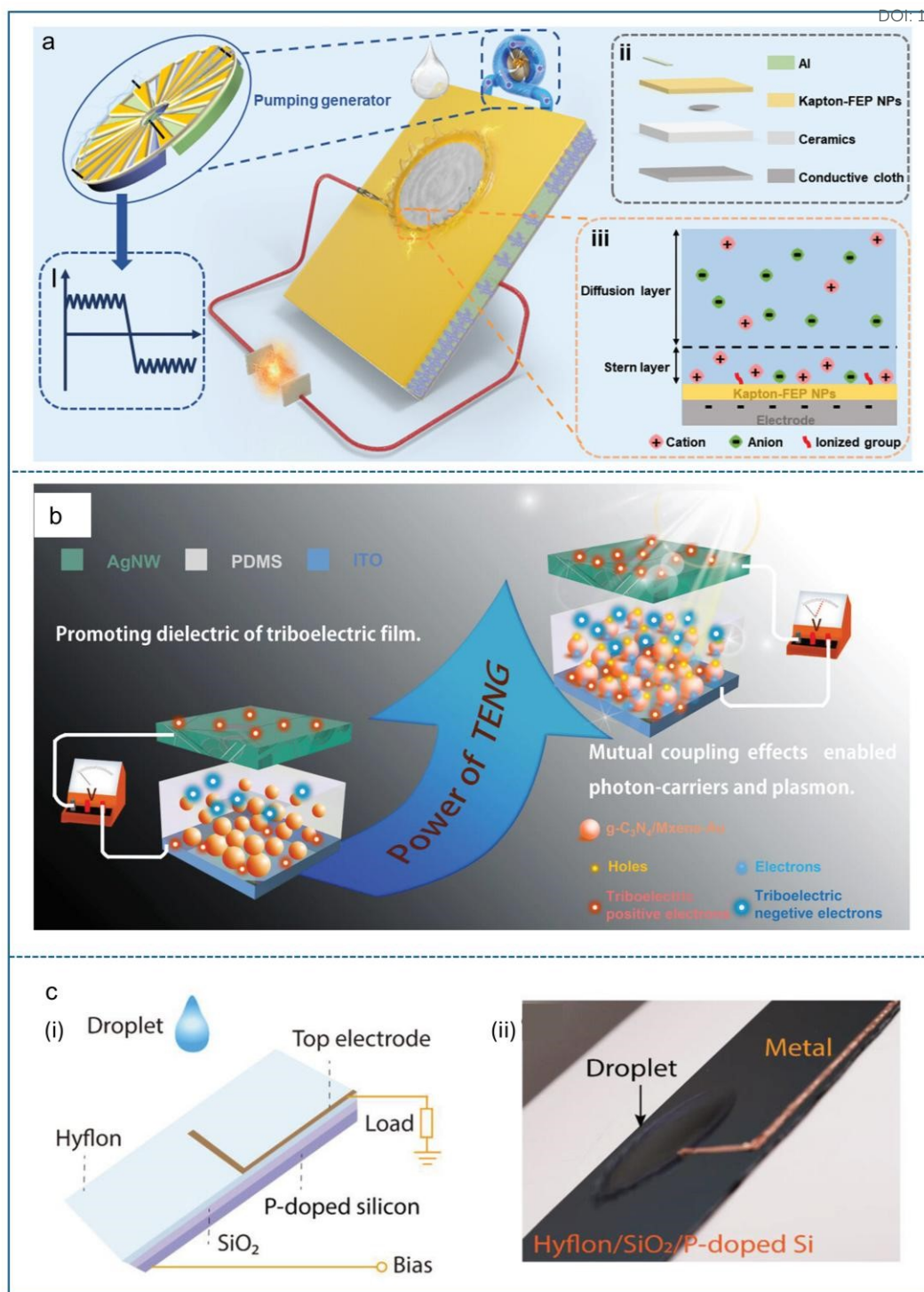
Figure 11. a) Externally charge-pumped liquid–solid TENG. Reproduced with permission. 222 Copyright 2024, Wiley-VCH GmbH. b) enhance TENG performance through charge trapping facilitated by photon-induced carrier generation. 223 Copyright 2021, Wiley-VCH GmbH. c) field-effect-enhanced droplet electricity generator. 224 Copyright 2023, Wiley-VCH GmbH
