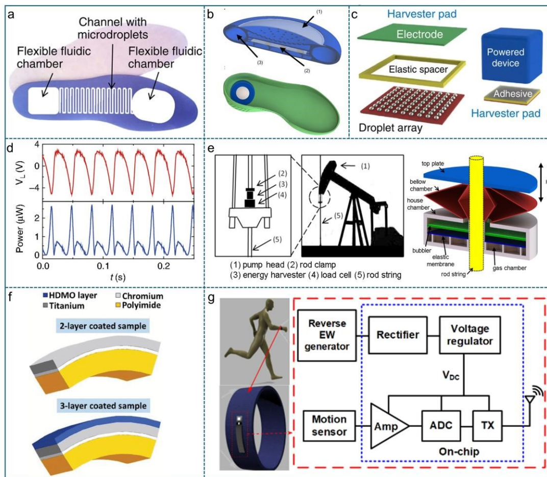
Figure 5. Application of REWOD as power sources. a) Schematic of a footwear embedded REWOD microfluidic energy harvester. Reproduced with permission. 34 Copyright 2011, Springer Nature. b) Cross-section of a footwear-integrated energy harvester based on the bubbler approach. Reproduced with permission. 101 Copyright 2015, Springer Nature. c) A REWOD-based vibration harvester. Reproduced with permission. 34 Copyright 2011, Springer Nature. d) Experimental results: voltage drop and instantaneous power with time for the case of a 14 droplets REWOD system. Reproduced with permission. 35 Copyright 2013, Springer Nature. e) (i) Schematics of oil pump and the possible location where to place the bubbler; (ii) The schematics of
