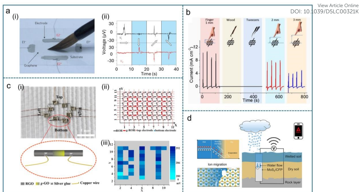
Figure 26. Applications for self-powered devices. a) (i) Photo of handwriting with a brush on graphene between four electrodes: E1 + , E1 - , E2 + and E2 - . a) (ii) The stroke directions by the drawing potential between electrodes can be sensed based on generated voltage signal. Reproduced with permission. 274 Copyright 2014, Springer Nature. b) Schematic of transpiration energy power generator for water seepage early warning system. Reproduced with permission. 382 Copyright 2023, American Chemical Society. c) (i) The units “0” and “1” can be integrated into the textile by random permutation and combination. Four information units are integrated into a piece of textile. c) (ii) Schematic of array of information storage units. c) (iii) Based on different voltage signal, the units are showing the logo of “BIT”. Reproduced with permission. 383 Copyright 2017, Elsevier. d) Generated streaming current with different objects and the changed position of fingers. Reproduced with permission. 354 Copyright 2018, Elsevier.
