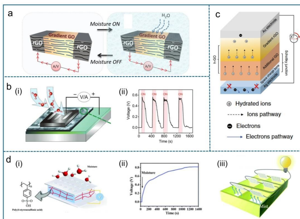
Figure 23. Application of moisture energy generator. a) Schematic of moisture-electric conversion cycle. The arrows represent induced voltage and current while moisture is in present and absence. Reproduced with permission. 354 Copyright 2018, Elsevier. b) (i) Schematic of \text{TiO}_2 based moisture energy generator generating electricity while harvesting moisture in the environment. b) (ii) Voltage generated in response to the 85% RH level. Reproduced with permission. 355 Copyright 2018, Wiley. c) Schematic of asymmetric sandwich structure of moisture energy generator. The feed layer with additional GO supplements the depletion of ions in the gradient rGO, and the special electrode/h-GO interface blocks the free electrons from passing through h-GO and regulates their flow direction, which greatly promotes the electrical output. Reproduced with permission. 356 Copyright 2019, Royal Society of Chemistry. d) (i) Schematic of PMEG, which consists of PSSA membrane between two gold electrodes. The upper electrode is manufactured with holes for efficient moisture access. d) (ii) The generated output voltage on a single 1 \times 1 \text{ cm}^2 PSSA membrane under constant moisture. d) (iii)
