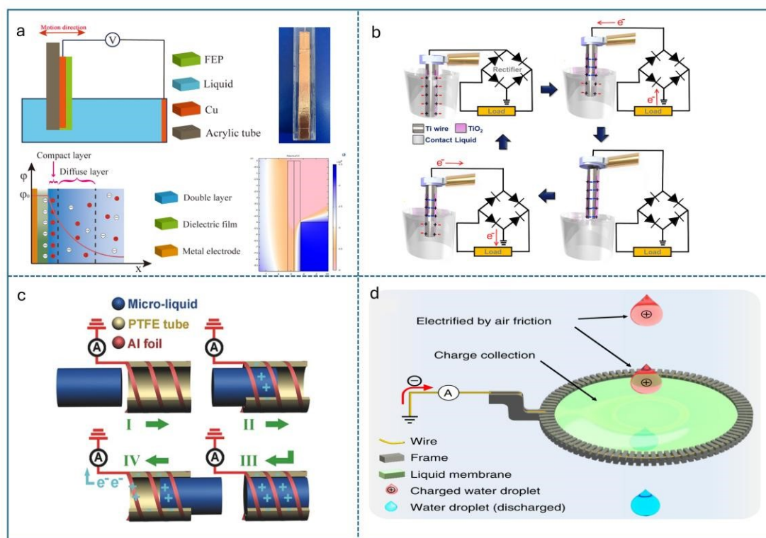
Figure 18. Applications of Liquid-Based TENGs in Sensors. a) Detection and classification of microplastics using deep learning integrated with liquid-based TENG technology. Reproduced with permission. 155 Copyright 2023, American Chemical Society. b) Working mechanism of \text{TiO}_2 -based liquid-solid Triboelectric nano-sensor for catechin detection. Reproduced with permission. 255 Copyright 2020, Elsevier. c) Working mechanism of capillary-tube triboelectric nanogenerator. Reproduced with permission. 256 Copyright 2018, Wiley-VCH GmbH. d) Rainfall sensing: establishing an approximately linear relationship between rainfall intensity and the device's electrical output. Reproduced with permission. 29 Copyright 2019, Springer Nature.
