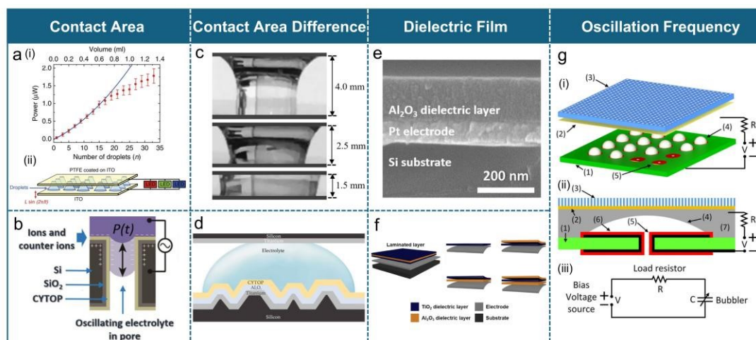
Figure 4. Strategies for improving electric output power. a) (i) Power versus the number of water bridges; the solid curve represents a parabolic fit, and data are presented as mean \pm standard deviation. (ii) Experimental setup for REWOD with a droplet array. Reproduced with permission. 35 Copyright 2013, Springer Nature. b) Working mechanism of high surface area REWOD energy harvesting under pulsating pressure, leading to AC voltage generation. Reproduced with permission. 98 Copyright 2022, Elsevier. c) Video freeze shots showing three stages of the electrolyte between electrodes during modulation, with electrode distance of 4 mm, 2.5 mm, and 1.5 mm. Reproduced with permission. 99 Copyright 2021, Springer Nature. d) Representative cross-sectional view of a rough electrode model. Reproduced with permission. 48 Copyright 2022, Wiley. e) Field emission scanning electron microscope image of a fabricated atomic layer deposition film sample. Reproduced with permission. 100 Copyright 2017, Elsevier. f) Schematic diagram of laminated structures. Reproduced with permission. 36 Copyright 2021, Springer. g) (i) Conceptual design of the bubbler: (1) REWOD chip, (2) membrane, (3) top plate, (4) an array of bubbles, (5) an array of electrodes; (ii) Schematics of a simplified single-electrode device used in the experiment: (1) REWOD chip, (2) membrane, (3) top plate, (4) bubble, (5) metal electrode, (6) dielectric coating, and (7) conductive liquid; (iii) Equivalent electrical circuit of the single-electrode device. Reproduced with permission. 101 Copyright 2015, Springer Nature.
