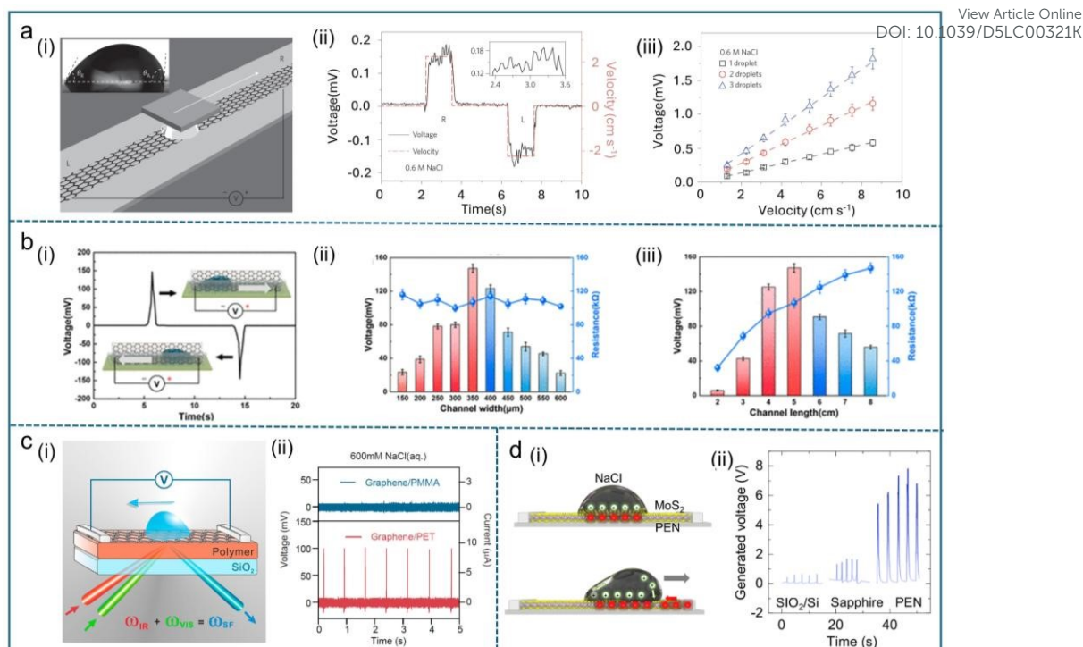
Figure 21. Application of droplet energy generator. a) (i) The droplet slides on the graphene sheet drawn by Si wafer, generating a drag potential. a) (ii) Drawing a droplet from the left end of the graphene strip to the right end and back again generates a voltage of 0.15mV. The reversed droplet velocity will generate a negative output voltage. a) (iii) The voltage induced when moving one, two, and three droplets. The output voltage is proportional to the number of droplets. Reproduced with permission. 274 Copyright 2014, Springer Nature. b) (i) The voltage generated by a 0.6 M NaCl solution when it moves in a graphene microchannel. The voltage direction varies with the flow direction of the droplet. b) (ii - iii) The output voltage of the graphene microchannel device changes at different channel widths and heights. Reproduced with permission. 334 Copyright 2022, American Chemical Society. c) (i) The droplet energy generator consisted of graphene/polymer film on SiO 2 plate. c) (ii) The graphene/PET film can generate 100mV pulse voltage, while it is undetectable on the graphene/PMMA. Reproduced with permission. 336 Copyright 2018, American Chemical Society. d) (i) Mechanisms of electricity generation while the droplet sliding on MoS 2 film. d) (ii) Voltage generated while MoS 2 film underlying on different substrates. Reproduced with permission. 339 Copyright 2020, Elsevier.
