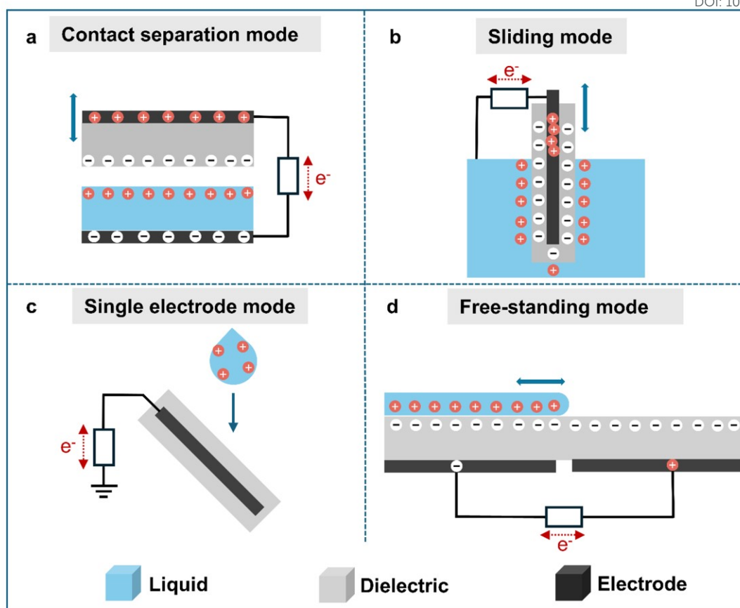
Figure 8. Basic modes of operation. (a) Contact-separation mode, (b) Sliding mode, (c) Single-electrode mode (d) Free-standing mode TENGs, respectively. Blue bidirectional arrows indicate the periodic mechanical motion. Red bidirectional arrows labeled "e - " represent the cyclic electron flow in the external circuit that changes direction during different phases of the mechanical cycle.
