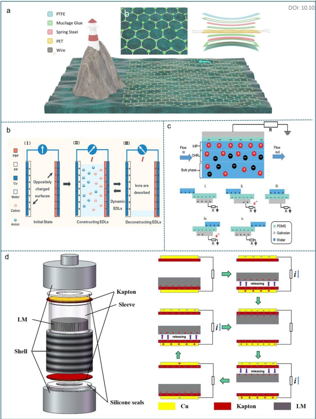
Figure 16. Bulk liquid based generator. a) Illustration of the OS-TENG structure and its potential for large-scale ocean wave energy harvesting. Reproduced with permission. 249 Copyright 2020, Elsevier. b) Asymmetric plate structure of the dielectric layer-based TENG. Reproduced with permission. 185 Copyright 2023, Wiley-VCH GmbH. c) Schematic of liquid metal-TENG harvesting energy through continuous water flow in and out. Reproduced with permission. 250 Copyright 2023, Wiley-VCH GmbH. d) Liquid-metal-based TENG optimized for low-frequency and multidirectional vibrations. Reproduced with permission. 184 Copyright 2021, Frontiers Media S.A.
