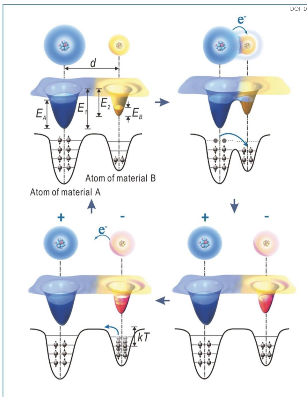
Figure 7. Electron-cloud-potential-well model. Reproduced with permission. 199 Copyright 2018, Wiley-VCH GmbH.
