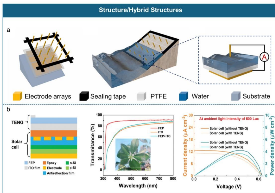
Figure 14. a) Wave Energy Harvester Utilizing a liquid-solid TENG Planar Array. Reproduced with permission. 244 Copyright 2021, Elsevier. b) Stacked Configuration of liquid-solid TENG and Solar Cell. Reproduced with permission. 245 Copyright 2023, Wiley-VCH GmbH.
