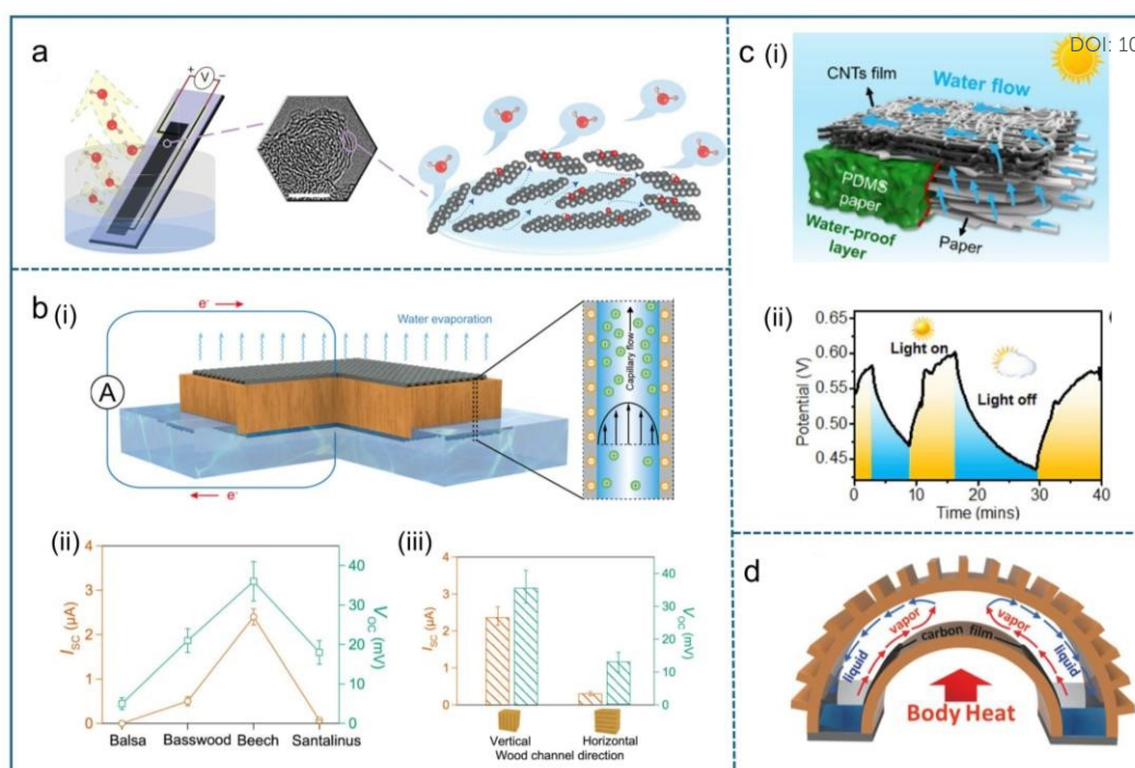
Figure 24. Applications of evaporation energy generator. a) Schematic of setup for harvesting energy from water evaporation through CB film. Reproduced with permission. 353 Copyright 2017, Springer Nature. b) (i) Schematic of the electricity generation induced by evaporation in a piece of wood. The microchannels of the wood piece are vertically aligned. When water flows in the microchannels, the inner surfaces of the channel are negatively charged, resulting in a positively charged flow. b) (ii - iii) Output voltage and current of different wood species and wood channel direction. Reproduced with permission. 364 Copyright 2020, American Chemical Society. c) (i) Schematic of solar-driven evaporator using a bilayer carbon nanotube/cellulose paper structure. c) (ii) Under solar irradiation, the electrical output enhanced compared to the dark environment. Reproduced with permission. 372 Copyright 2020, Elsevier. d) Schematic of self-powered wearable wristband. While the DI water evaporated driven by body heat, the porous carbon membrane harvesting the energy from evaporation to electricity. Reproduced with permission. 374 Copyright 2018, Wiley.
