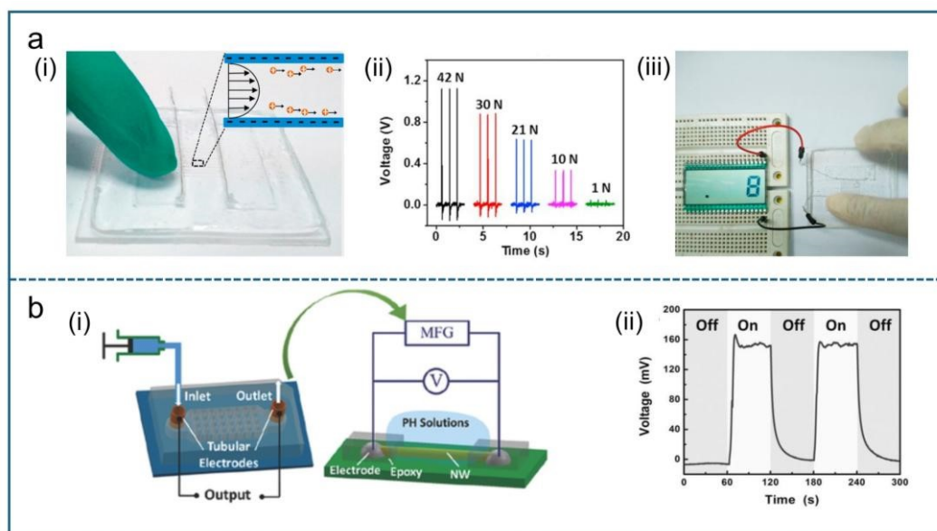
Figure 25. Applications of microfluidic energy generator. a) (i) Schematic of flexible MFNG consists of ten microchannels. The width of each channel is 100\ \mu\text{m} . a) (ii) The voltage generated by MFNG at different external forces. a) (iii) Photo of LCD powered by MFNG directly. Reproduced with permission. 375 Copyright 2016, Elsevier. b) (i) Schematic of microfluidic nanogenerator with porous patterned structure in the microchannel, where the microfluidic nanogenerator supplied energy to a single NW based pH sensor. b) (ii) Voltage generated from microfluidic when a 1\ \mu\text{M} KCl solution flows through the device at 0.4\ \text{mL/min} . Reproduced with permission. 31 Copyright 2015, Wiley.
