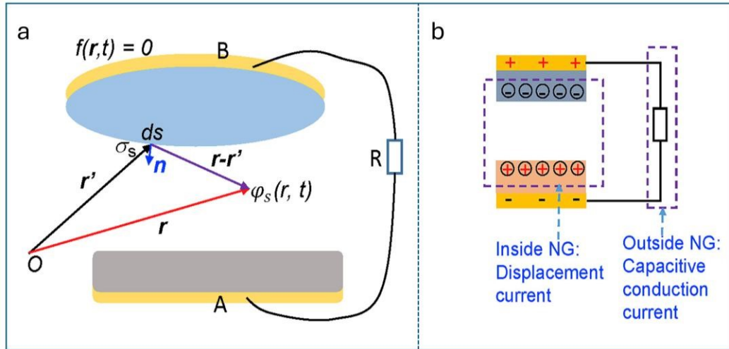
Figure 7. a) A schematic illustration of a TENG connected to an external load, along with the corresponding coordinate system used for mathematical modeling and analysis. b) Schematic showing Displacement current and conduction current in TENG. Reproduced with permission. 165 Copyright 2020, Elsevier.
