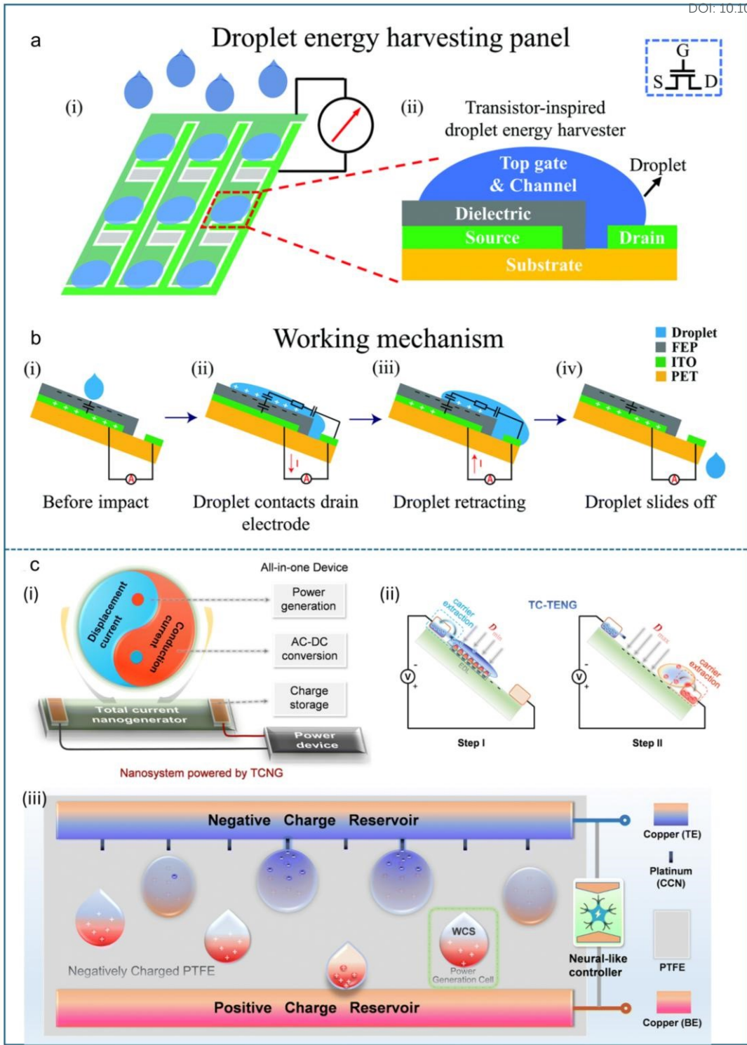
Figure 13. (a) Schematic of the droplet energy harvesting (DEH) panel and its transistor-inspired unit cell. Reproduced with permission. 240 Copyright 2022, Royal Society of Chemistry (b) Working mechanism illustrating charge transfer from source to drain upon droplet spreading, followed by charge recovery as the droplet retracts and exits. Reproduced with permission. 240 Copyright 2022, Royal Society of Chemistry (c) (i) Conceptual framework of TCNG systems integrating power generation and management. (ii) Representative charge induction steps in TC-TENG operation. (iii) Bioinspired TC-TENG design featuring dual charge reservoirs and neural-like
