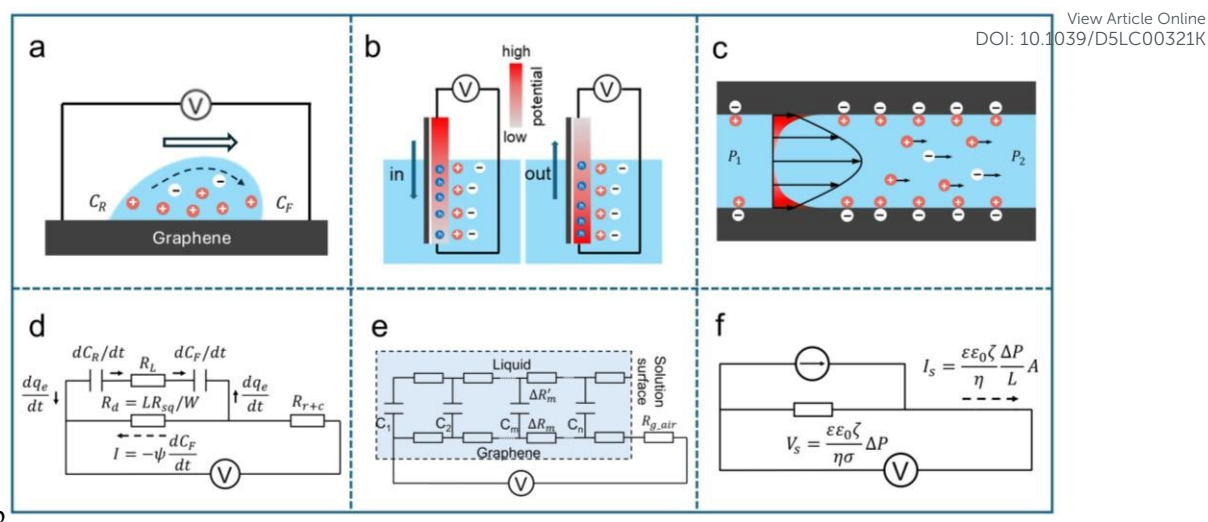
Figure 19. Basic working principles of electrokinetic energy conversion. a) Schematic illustration of pseudocapacitance formed at front and rear edge of moving droplet inducing the potential difference. b) Schematic of adsorption (left) and desorption (right) of ions on the graphene surface forming EDL and its boundaries, during insertion and withdrawal processes. The illustration also depicts the induced potential difference and the hole concentration gradient within the graphene sheet. c) Schematic of electrokinetic streaming current/potential generated through pressure driven electrolyte flow within micro/nano channels. The positive and negative charges are indicated with red and white circles. d) Equivalent circuit of drawing potential. e) Equivalent circuit of waving potential. f) Equivalent circuit for streaming potential.
