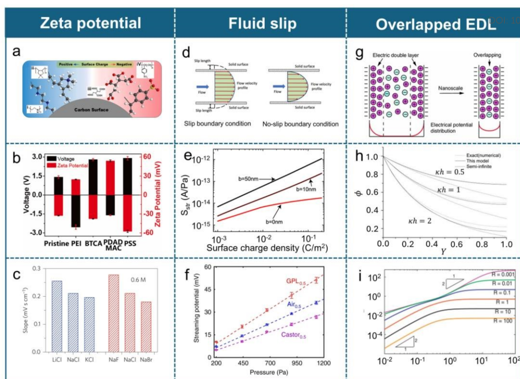
Figure 20. Strategies to improve electrical output. a) Schematic of different molecules modification on carbon particles. Reproduced with permission. 284 Copyright 2019, Elsevier. b) Streaming potential generated on different PSS, BCTA, PEI, PDADMAC modified surface with different zeta potential levels. Reproduced with permission. 284 Copyright 2019, Elsevier. c) The waving potential generated across electrolyte with different ion radius. Reproduced with permission. 274 Copyright 2014, Springer Nature. d) Schematic of velocity field near the interface with no-slip boundary condition (left) and Navier-slip boundary condition (right) Reproduced with permission. 327 Copyright 2021, Elsevier. e) Increasing the slip length to from 0 nm to 50 nm could theoretically boost the maximum conversion efficiency. Reproduced with permission. 300 Copyright 2008, Wiley. f) The SLIPS can overperforming the generated streaming potential compared to flat and superhydrophobic surfaces with same pattern. Reproduced with permission. 310 Copyright 2018, Springer Nature. g) The overlapped EDL can significantly enhance the counterions concentration at center of channel. Reproduced with permission. 328 Copyright 2012, Springer Nature. h) As the ratio between channel height and Debye length increase, the dimensionless potential significantly reduced. Reproduced with permission. 322 Copyright 2010, American Institute of Physics. i) Variation of dimensionless streaming potential influenced by synergistic effect of dimensionless EDL thickness and ionic Peclet number. Reproduced with permission. 323 Copyright 2013, Elsevier.
