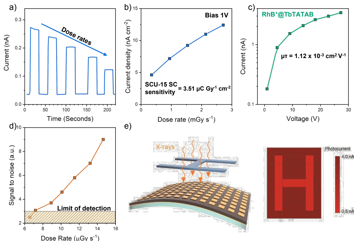
Figure 5: Summary of direct X-ray characterisation of MOFs. a) The photocurrent of SCU-15 SC decreased versus time under different dose rates from 2.75 to 0.53 mGy/s. Reproduced with permission from [80]. b) X-ray induced current response with increasing dose rate of SCU-15 SC, and maximum sensitivity measurement. Reproduced with permission from [80]. c) Mobility–lifetime product of best performing mobilities demonstrated in a MOF direct X-ray detector (RhB+@TbTATAB) derived from the photoconductivity curves. Reproduced with permission from [77]. d) X-ray dose-dependent signal-to-noise ratio of the Ni-DABDT detector, with limit of detection highlighted. Reproduced with permission from [69]. e) Schematic structure of X-ray prototype imaging device based on the Ni-DABDT material and X-ray imaging of an aluminium bulk with the letter “H” pattern. Reproduced with permission from [69].
