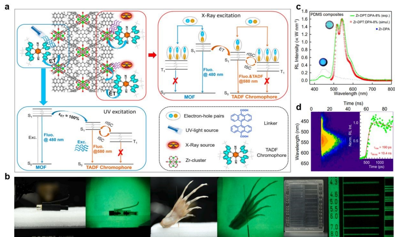
Figure 4: (a) Illustration of the radioluminescence mechanism, with highly efficient energy transfer from the Zr-fcu-BADC-MOF to the TADF chromophore, under ultraviolet-light irradiation. The acronyms are: ET (energy transfer); ISC (intersystem crossing); rISC (reverse intersystem crossing). Reproduced with permission from [50]. (b) The developed Pb-MOF scintillating film, applied in a simple X-ray imaging system, on a commercial lighter (left), bullfrog claw (middle), and line pairs card (right), under 50 kV X-ray irradiation. The spatial resolution achieved was 5.5 lp mm -1 . This value is superior to 1.1 lp/mm obtained using another composite film of organic anthracene scintillator. Reproduced with permission from [51]. (c) Experimental radioluminescence spectrum of nanocomposites with hetero-ligand Zr-DPT:DPA-8% (red) and homo-ligand Zr-DPA nanocrystals (blue), with PDMS as the host polymer matrix. The simulated radioluminescence spectrum is also shown (green). (d) 2D map of composite scintillation emission. Inset: Scintillation pulse with average decay time of 10.4 ns. Reproduced with permission from [52].
