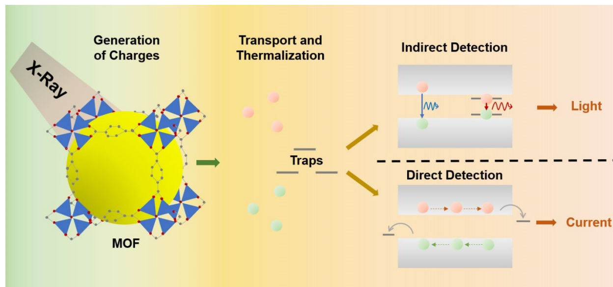
Figure 1: Free charges are generated by the interaction of the X-ray with the MOF. For indirect detection (scintillation), the incident X-rays are down-converted to photons which are collected by a photodetector. For direct detection, the incident X-rays are directly converted into current which are collected at the electrodes.
