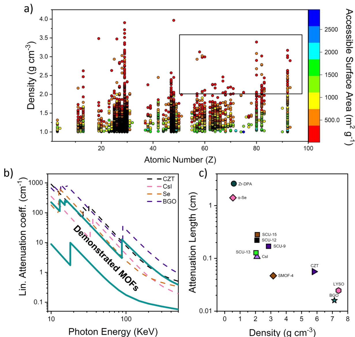
Figure 2: Comparison of MOF X-ray detection attenuation properties. a) Synthetic versatility and potential of high-throughput database screening of MOFs for X-ray detection demonstrated using the Cambridge Structural database (non-disordered MOF subset). The plot shows the atomic number, density and accessible surface area of MOFs, with an area highlighted for possible high attenuation MOFs. b) Linear attenuation coefficients of MOFs used for X-ray detection and commercial materials from 10 to 500 keV. c) Comparison of density and attenuation length required for 100% attenuation at 100 keV of MOFs used in X-ray detection and commercial materials.
