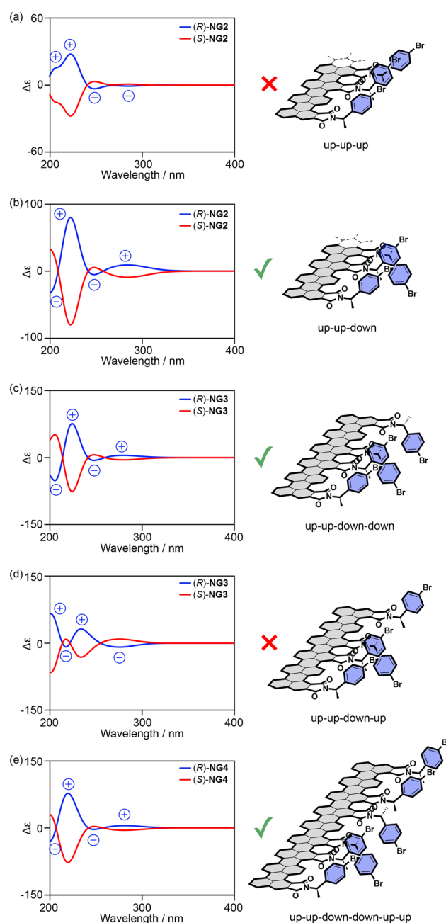
Fig. 18 (a)–(e) Calculated CD spectra of model edge structures with (a) up-up-up, (b) up-up-down, (c) up-up-down-down, (d) up-up-down-up, and (e) up-up-down-down-up-up orientations (ref. 71). Copyright 2024 Wiley-VCH.
