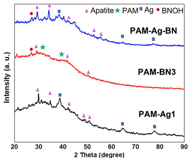
Fig. 10 XRD pattern of the PAM-Ag1, PAM-BN3 and PAM-Ag-BN hydrogel samples showing specific apatite peaks.
