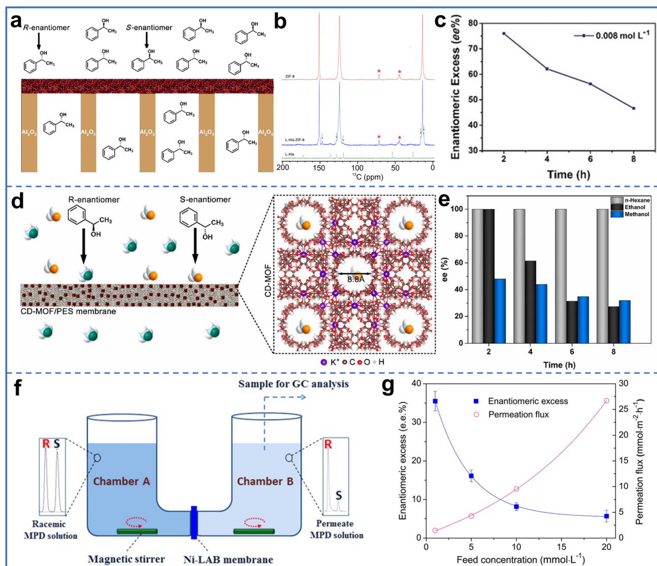
Fig. 11 (a) Schematic of the L-His-ZIF-8 membrane separating racemic 1-phenylethanol. (b) ^{13}\text{C} CPMAS NMR spectra of ZIF-8, L-His-ZIF-8, and L-His. (c) Enantiometric excess with time in separation of racemic 1-phenylethanol by L-His-ZIF-8 membrane. Reproduced with permission from ref. 19. Copyright 2018, Wiley-VCH. (d) Schematic of the separation of the 1-phenylethanol racemic mixture by CD-MOF/PES MMM. (e) Effect of solvents on separation of 1-phenylethanol racemates by MMMs. Reproduced with permission from ref. 53. Copyright 2021, Elsevier B.V. (f) Schematic of the separation of racemic MPD at low temperature through a \text{Ni}_2(\text{L-asp})_2(\text{bipy}) membrane. (g) Enantiometric excess and permeation flux with feed concentrations at 30 °C in the separation of racemic MPD by \text{Ni}_2(\text{L-asp})_2(\text{bipy}) membrane. Reproduced with permission from ref. 83. Copyright 2013, Wiley-VCH.
