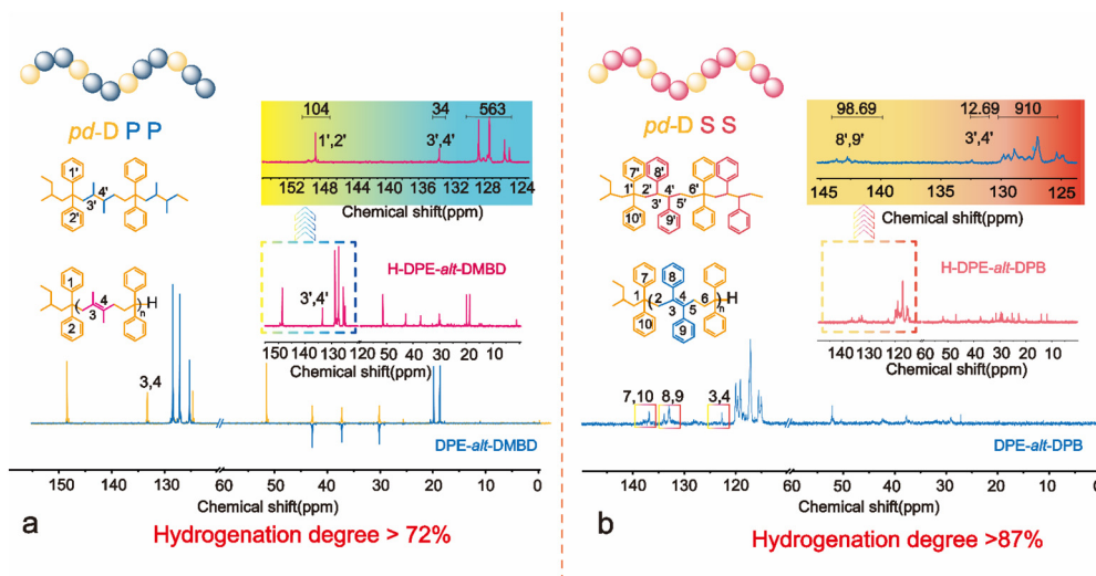
Fig. 3 IG- 13 C NMR spectra of alternating polymers and periodic polymers: (a) for the copolymer of DPE with DMBD and (b) for the copolymer of DPE with DPB.
