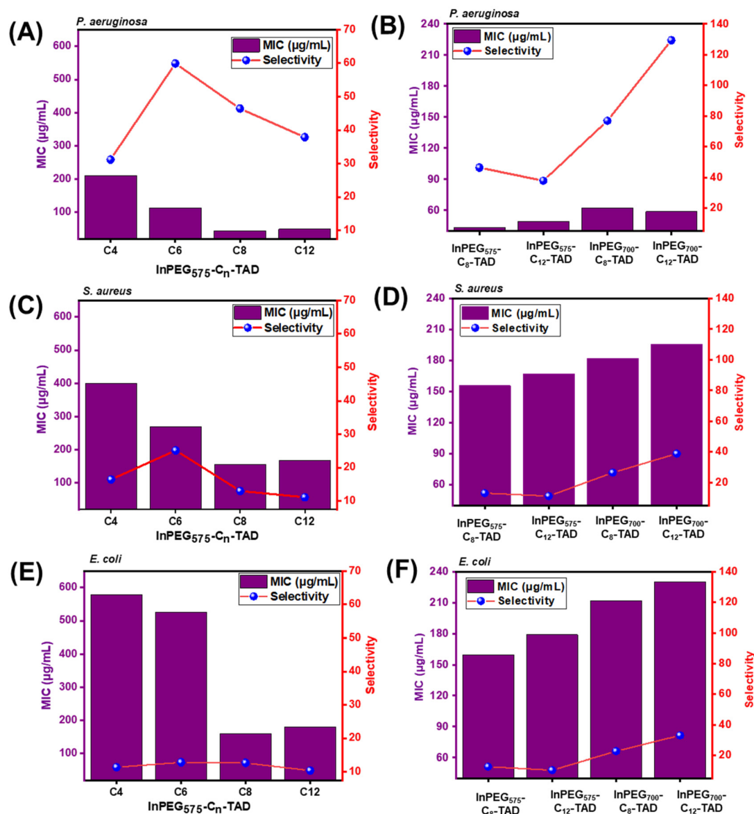
Fig. 6 Graphical representation of the structure–antimicrobial activity–hemolytic activity relationship of different PEG derivatives: (A), (C) and (E) represent the effect of different alkyl chain lengths on the antimicrobial activity and selectivity of the InPEG 575 -Cn-TAD polymer series against P. aeruginosa , S. aureus and E. coli , respectively; (B), (D) and (F) represent the effect of PEG chain length on antimicrobial activity and selectivity against P. aeruginosa , S. aureus and E. coli , respectively (the two best-performing polymers InPEG 575 -C 8 -TAD and InPEG 700 -C 12 -TAD were chosen for comparison).
