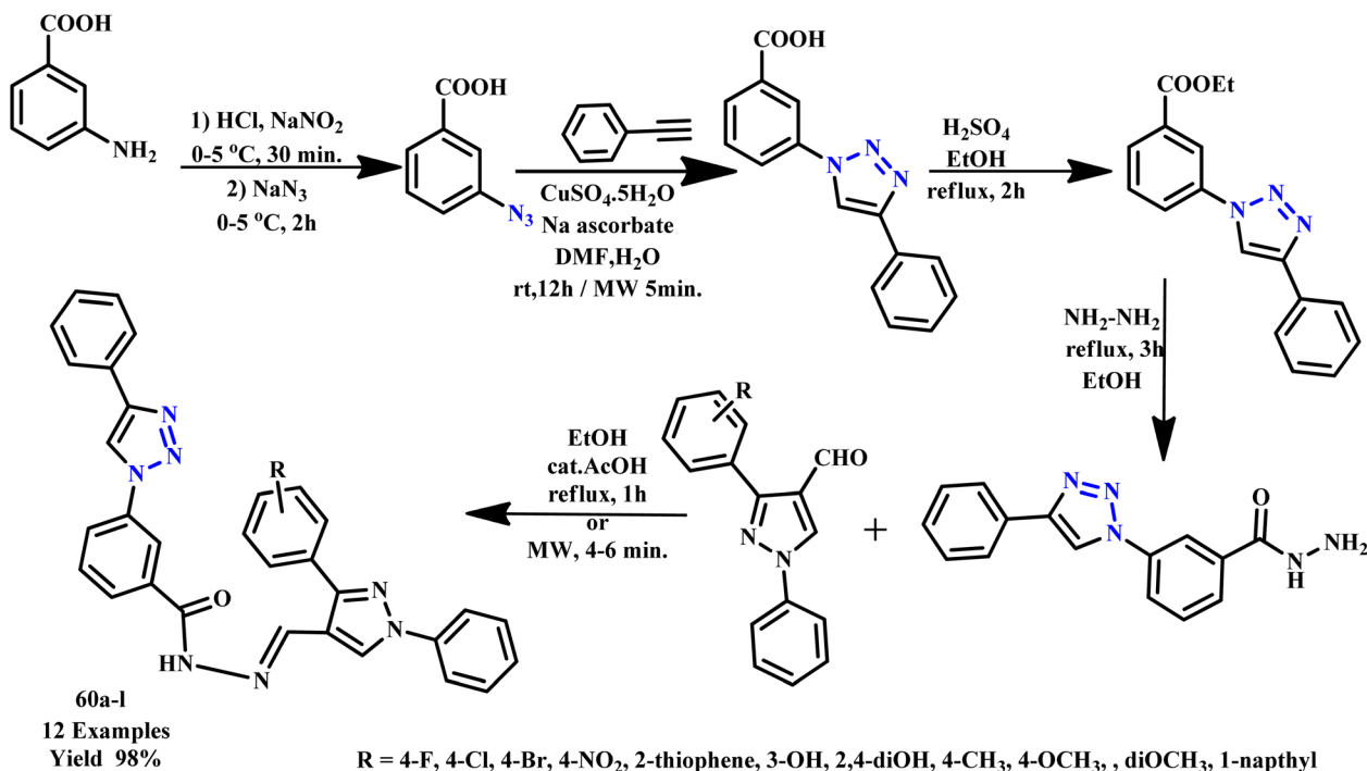
Scheme 49 Synthetic route for 3-(4-phenyl-1 H -1,2,3-triazol-1-yl)benzohydrazide derivatives (60a–l). 92
