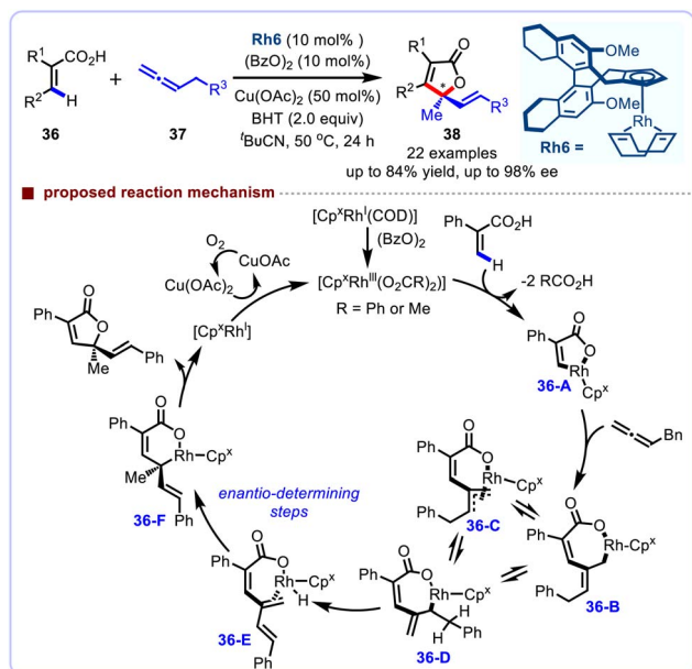
Scheme 14 \text{Cp}^x\text{Rh(III)} -catalyzed asymmetric alkenyl C–H functionalization of acrylic acids.
