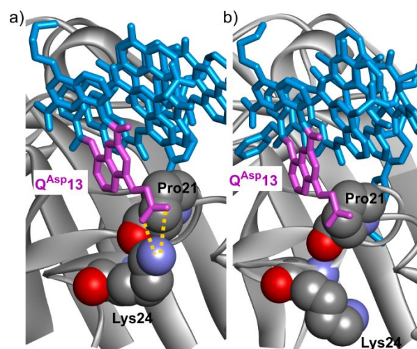
Fig. 7. Solid state structures of HCAII in complex with: a) 2 , b) 20 . The protein is shown in gray ribbon representation except P21 and Lys24, which are in space filling representation. The foldamer is shown in blue stick representation except the residue in position 13, which is colored in purple. Hydrogen bonds are indicated as yellow dashed lines.
