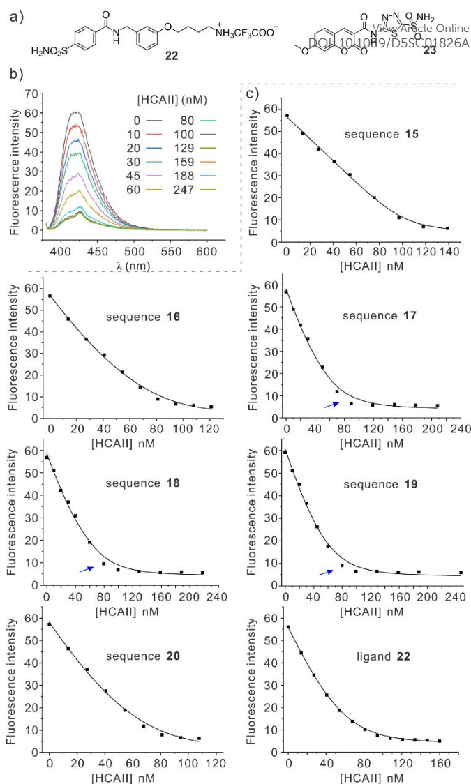
Fig. 8. a) Structural formula of HCAII ligand 22 and of fluorescence probe 23 used in the competition assay. b) Changes in fluorescence spectra (380 nm – 600 nm) upon HCAII titration of sequence 19 . [ 19 ] = [ 23 ] = 50 nM; c) Experimental (■) and calculated values using a 1:1 binding isotherm (-) of fluorescence intensity of sequences 15-20 and 22 titrated with HCAII. [competing species] = [ 23 ] = 50 nM. Note that the curve fitting is shown at one wavelength (419 nm) as an illustration but that the K_D values (Table 1) were calculated by simultaneously fitting data recorded in the 380-600 nm range. Blue arrows point to a systematic error discussed in the text.
