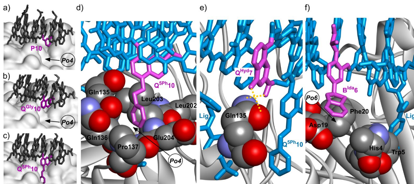
Fig. 6. Solid state structures of HCAII in complex with: a) 1 , b) 2 , c) 3 , d,e) 16 , f) 20 . In a)–c), the protein is shown as a white soft surface and the foldamer is shown in stick representation in gray except the residue in position 10 colored in purple. In d)–f), the protein is shown in gray ribbon representation except relevant amino acids which are in space filling representation. The foldamer is shown in blue stick representation except the residue in position 10 in d), the residue in position 7 in e) and the residue in position 6 in f), which are colored in purple. Hydrogen bonds are indicated as yellow dashed lines. Pockets Po4 and Po6 are defined in Fig. 4
