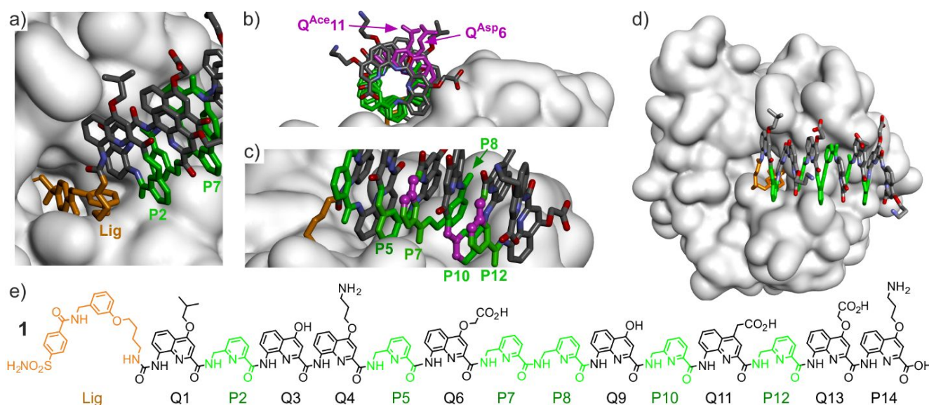
Fig. 2. a), b), c) and d) show different views of the solid state structure of the complex between HCAII and AOF 1 . 3 Only the surface of the protein is shown. The foldamer is shown in stick representation. Pyridine units (P) are shown in green and the HCAII ligand is shown in gold. In b), two residues of interest are shown in purple. In c) three carbon atoms of three P residues are shown in purple balls. These carbons would belong to the additional benzenic ring when implementing a P->Q mutation at these positions. Hydrogen atoms have been omitted for clarity. e) Structural formula of 1 .
