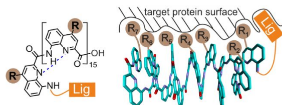
Fig. 1. Chemical formula (left) of a hexadecaamide of 8-amino-2-quinolinecarboxylic acid bearing a protein ligand (Lig) at the N terminus and biogenic-like side chains (R groups) in position 4. Schematic representation (right) of the helical structure of the hexadecaamide with some R groups interacting with a protein surface to which the ligand is also bound.
