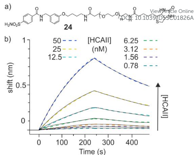
Fig. 9. a) Structural formula of biotinylated HCAII ligand 24 . b) BLI sensorgrams (black solid lines) of the titration of 24 immobilized on the streptavidin sensors at different HCAII concentrations. Calculated curves based on a 1:1 binding isotherm (colored dashed lines) fit with the measured values, yielding K_D = 38.2 nM.
