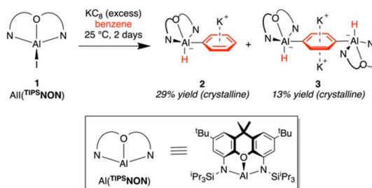
Scheme 2 Reduction of Al(TIPSNON) with excess KC_8 at room temperature to give benzene C–H activated products 2 and 3 .
