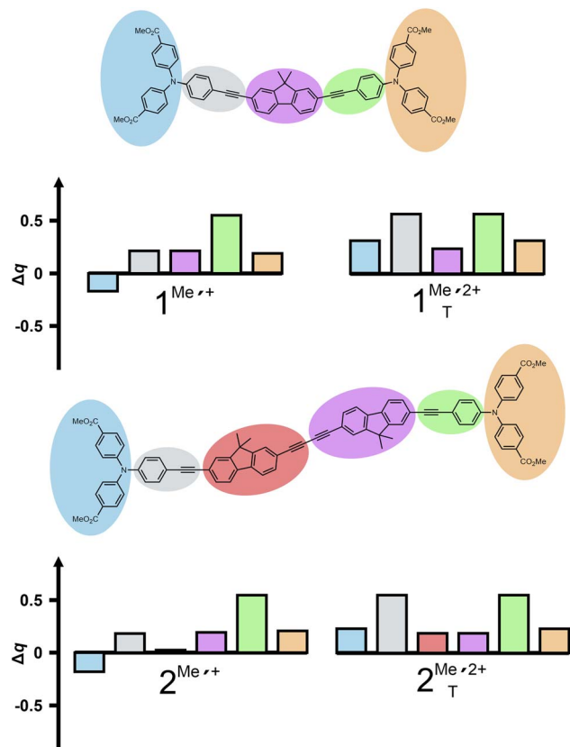
Fig. 5 Calculated electron density losses upon oxidation of model complexes 1^{Me'} and 2^{Me'} to their corresponding one- (left) and two-electron oxidized forms (triplet state), based on natural bond orbital (NBO) analysis. \Delta q refers to the charge difference of the respective molecular region of the radical monocations (left panels) and the respective dications in their triplet ground state (right panels) relative to the corresponding neutral state. The individual fragments are color-coded according to the graphical representation in the top panels.
