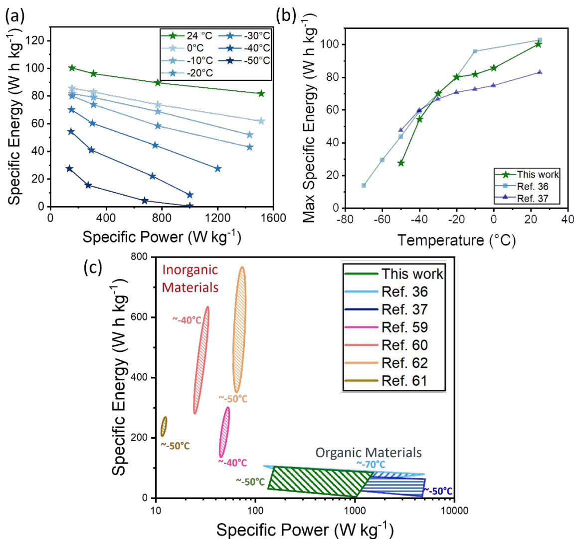
Figure 8 (a) Ragone plot of the dual-ion battery of this work at different temperatures from -50 ^{\circ}\text{C} to room temperature. (b) Maximum specific energy vs temperature plot for this work and two others. 36, 37 (c) Ragone plot of recent low-temperature batteries. 36, 37, 59-62 Organic batteries at low temperatures show a specific power that is roughly 3-10 times higher than inorganic ones at maximum specific energy.
