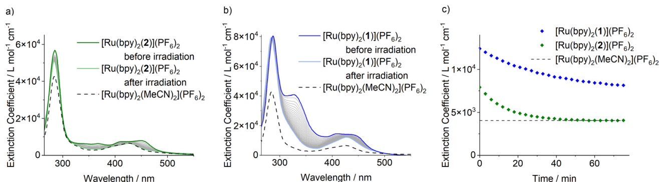
Fig. 2 (a) UV-vis absorption (10 μM, acetonitrile, 298 K) spectra of [\text{Ru}(\text{bpy})_2(2)](\text{PF}_6)_2 after irradiation at 365 nm for 75 minutes. From 0 minutes (dark green) to 75 minutes (light green). UV-vis absorption spectra of [\text{Ru}(\text{bpy})_2(\text{MeCN})_2](\text{PF}_6)_2 is shown through a dashed line. (b) UV-vis absorption spectra of [\text{Ru}(\text{bpy})_2(1)](\text{PF}_6)_2 (13 μM, acetonitrile, 298 K) after irradiation at 365 nm for 75 minutes. From 0 minutes (dark blue) to 75 minutes (light blue). UV-vis absorption spectra of [\text{Ru}(\text{bpy})_2(\text{MeCN})_2](\text{PF}_6)_2 is shown through a dashed line. (c) Extinction coefficient at 450 nm of [\text{Ru}(\text{bpy})_2(1)](\text{PF}_6)_2 and [\text{Ru}(\text{bpy})_2(2)](\text{PF}_6)_2 (acetonitrile, 298 K) during irradiation with 365 nm light for 75 minutes. [\text{Ru}(\text{bpy})_2(\text{MeCN})_2](\text{PF}_6)_2 is shown through a dashed line.
