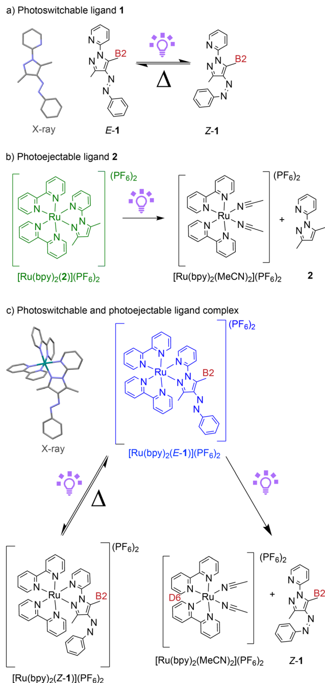
Fig. 1 (a) Photoswitchable ligand, 1 , and its UV light triggered photo-switching. (b) Ruthenium complex, [Ru(bpy) 2 ( 2 )](PF 6 ) 2 , containing non photoswitchable ligand 2 and its photoejection triggered by UV light. (c) Ruthenium complex, [Ru(bpy) 2 (E-1)](PF 6 ) 2 , containing photo switchable ligand 1 and its photoejection and photo isomerisation triggered by UV light. Chosen hydrogen environments are labelled in red.
