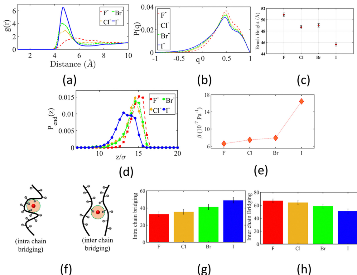
Fig. 24 (a) RDF of \{N(CH_3)_3\}^+X^- ( X = I^- , Br^- , Cl^- , and F^- ). (b) Probability distribution of the tetrahedral order parameter ( q ) of the solvating water of the \{N(CH_3)_3\}^+ moiety. (c) Variation of the height of the PMETA + brushes for the cases where the PMETA + brushes are screened by different halide counterions. (d) End chain monomer distributions of the PMETA + brushes. (e) Variation of the compressibility factor of the PMETA + brush system. In (b), (d), and (e), results are shown for the individual cases where the PMETA + brushes are screened by different halide counterions. (f) Schematic of two types of bridging interactions: intrachain bridging and interchain bridging. (g) Percentage of intrachain bridging undergone by the monomers of the PMETA + chains screened by different halide counterions. (h) Percentage of interchain bridging undergone by the monomers of the PMETA + chains screened by different halide counterions. All the parts of the figure have been reprinted with permission from Ishraaq, R.; Das, S., All-Atom molecular dynamics simulations of cationic polyelectrolyte brushes in the presence of halide counterions, Macromolecules , 2024, 57 (7), 3037–3046. Copyright (2024) American Chemical Society.
