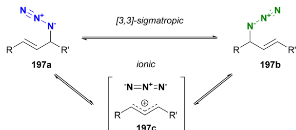
Fig. 14 Winstein rearrangement of allyl azides.
