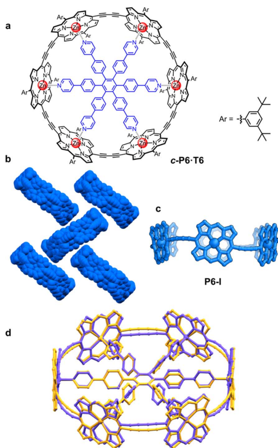
Fig. 1 (a) Drawing of a six-porphyrin nanoring with the template marked in blue, Ar = 3,5-di-tert-butylphenyl. (b) Fragment of the crystal structure of the previously reported, orthorhombic (Pccc) polymorph P6-I (CCDC: 860774). 6 (c) View of the molecular conformation of the nanoring in P6-I. Hydrogen atoms, template and aryl groups in (b) and (c) are omitted for clarity. (d) Comparison of the molecular geometry of c-P6·T6 from the published crystal structure of polymorph P6-I (purple) 6 and the gas-phase geometry from DFT calculations (BLYP35/6-31G*, yellow). 16
