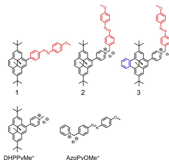
Fig. 3 Studied derivatives.
