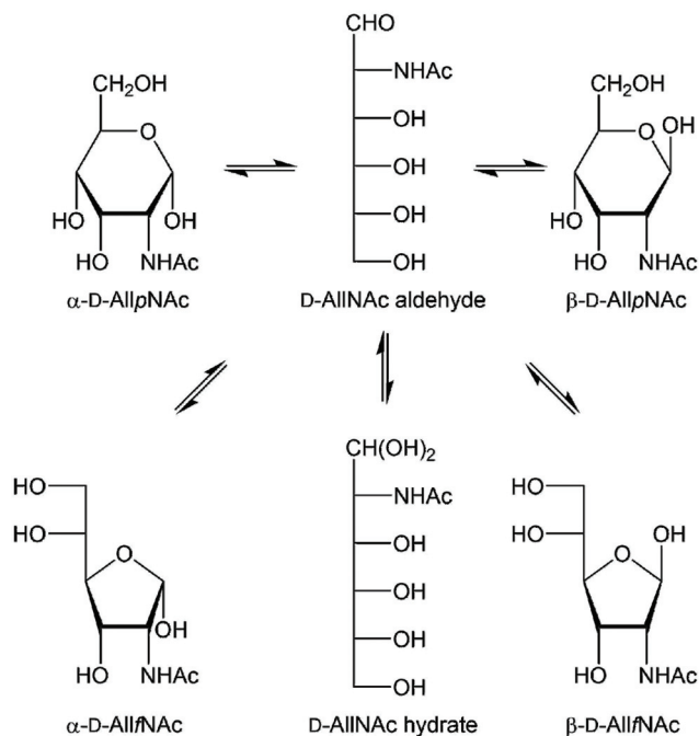
Scheme 1 Schematic of the equilibria of tautomeric acyclic and ring forms of N -acetyl- D -allosamine in water solution. The four different ring forms are readily observable by 1 H NMR spectroscopy.
