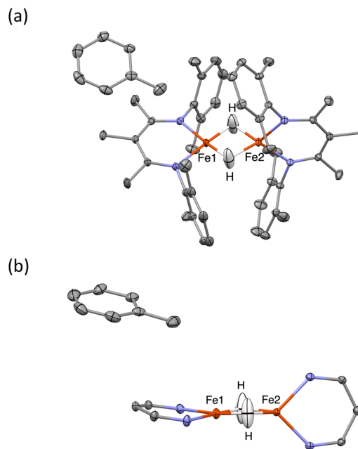
Fig. 5 Thermal-ellipsoid plots from the neutron crystal structure of 1-toluene , using 50% probability ellipsoids. (a) View along the C_2 axis. (b) View along the plane of Fe1, showing the different geometries of the sites. Diketiminato substituents are omitted for clarity.
